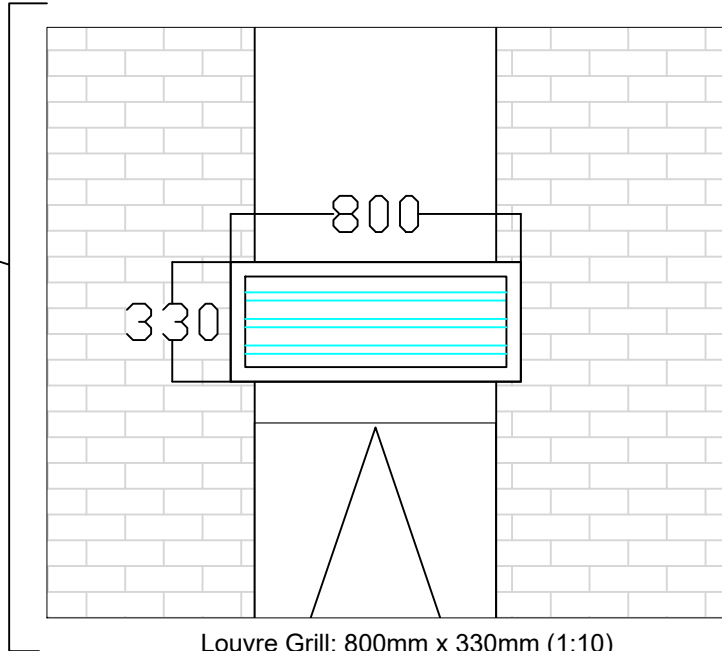
Louvre Grill: 800mm x 330mm (1:10) Material/Colour : Aluminium Natural Finish
