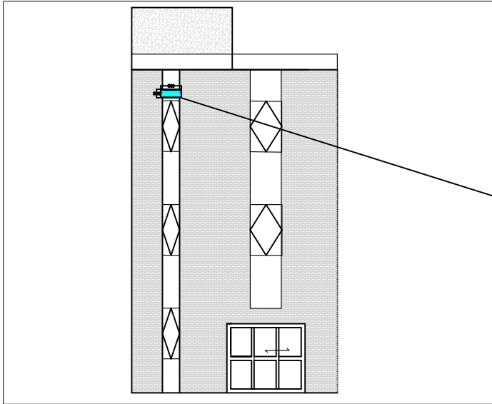
Proposed Elevation 4 (1:100)
