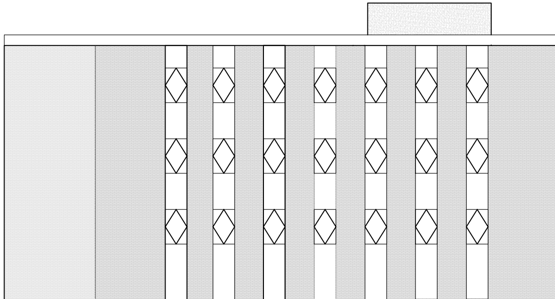
Existing Elevation 1 (1:100)
