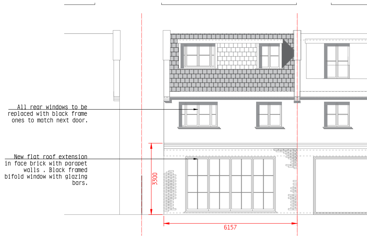
050.2 REAR ELEVATION AS PROPOSED
