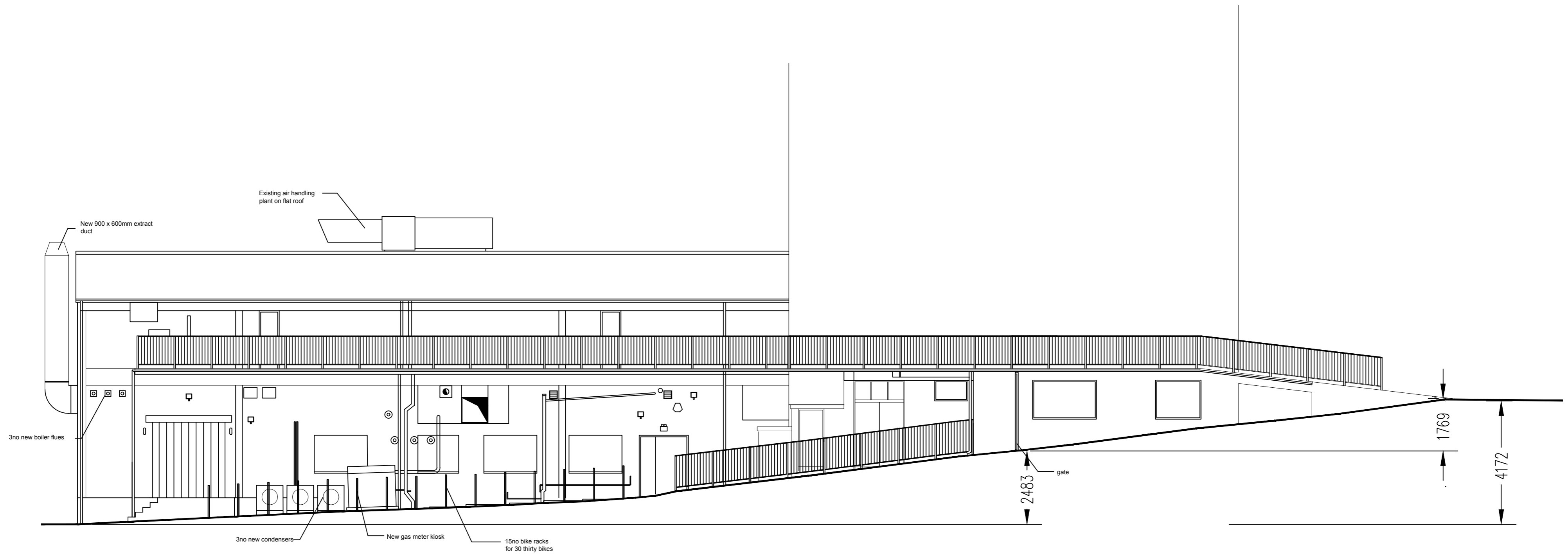
Proposed South Elevation
