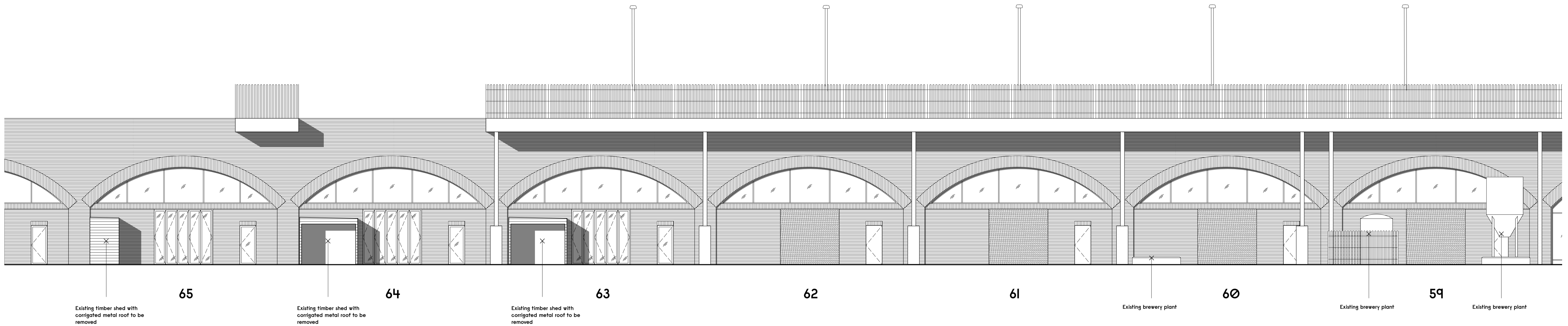
1 Existing Arches 59-65 Elevation A Scale: 1:100
