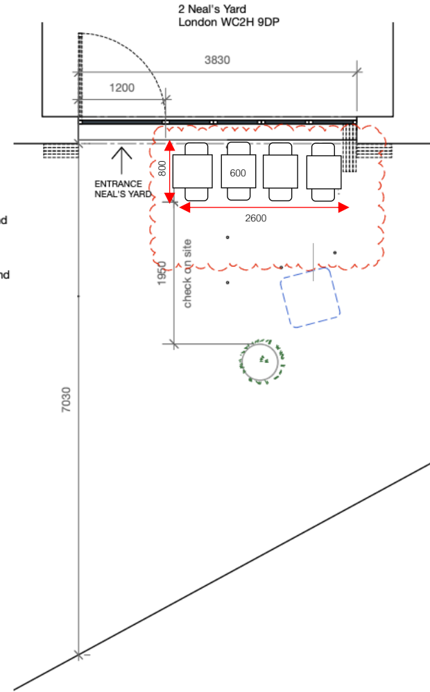
2 proposed plan outdoor seating Scale: 1:50
