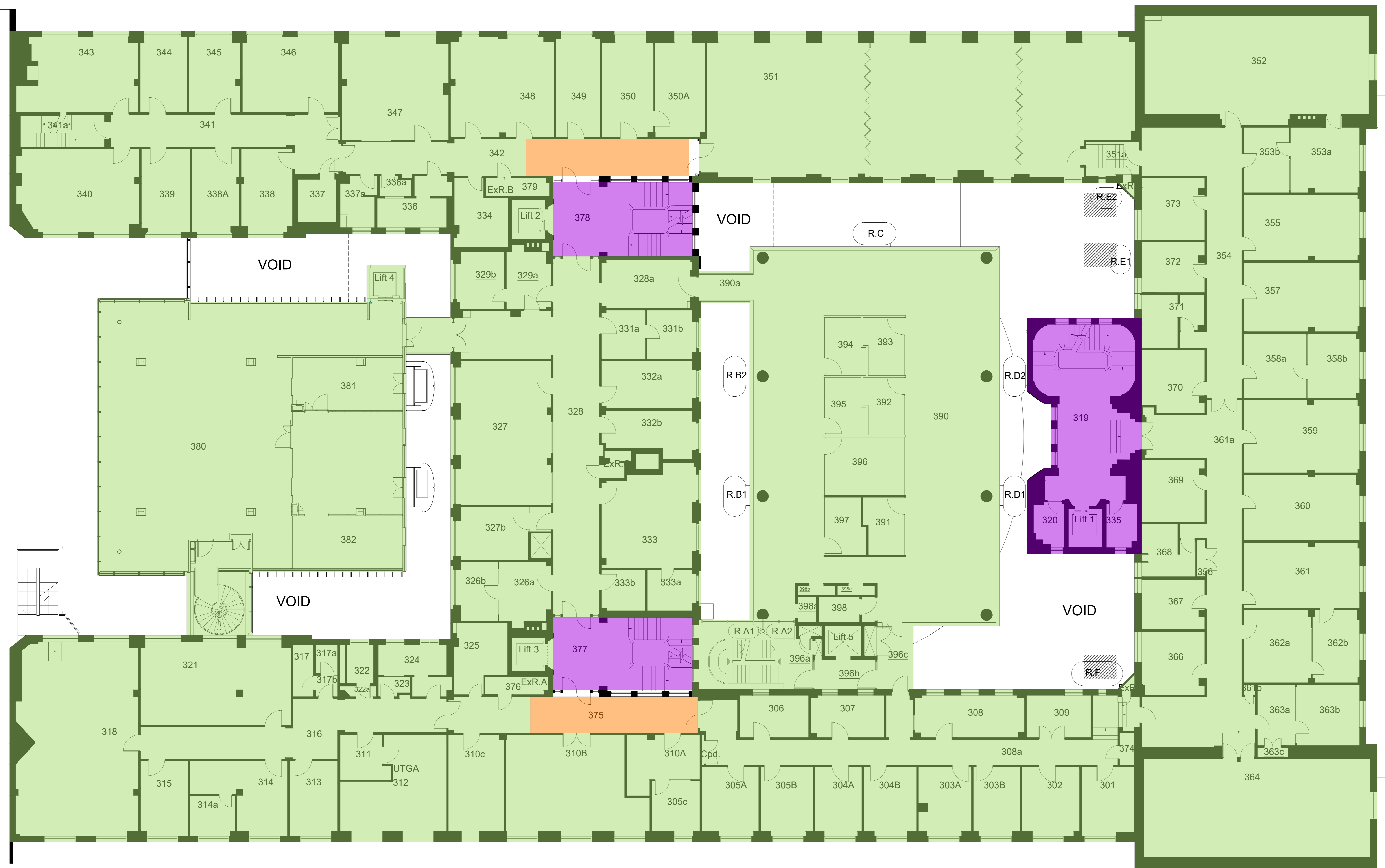
01 Level 03 - Plan - Conservation Strategy 08-2033 Scale = 1:100
