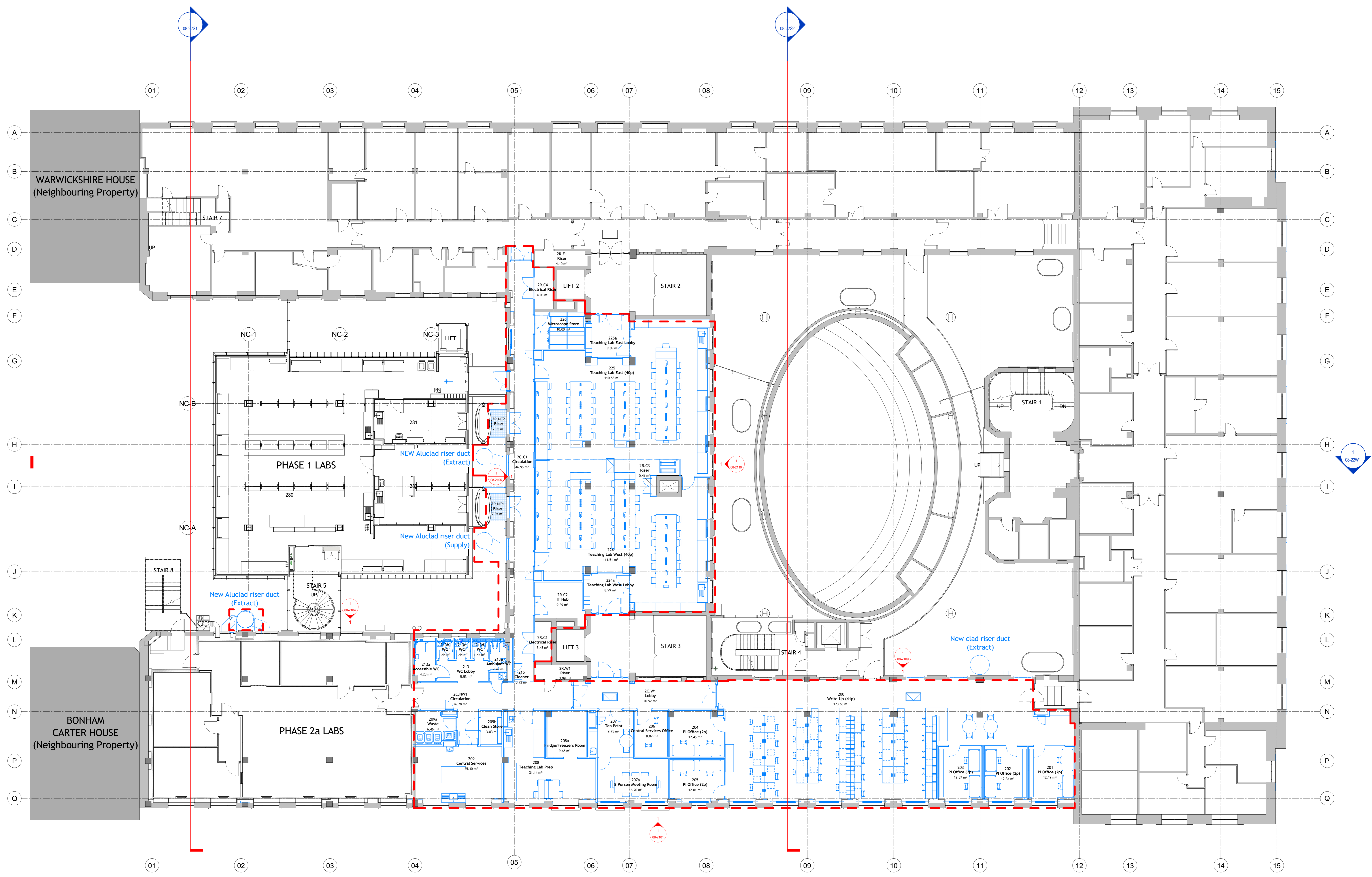
1 GA Plan - Planning - Level 2 Proposed 1 : 100
