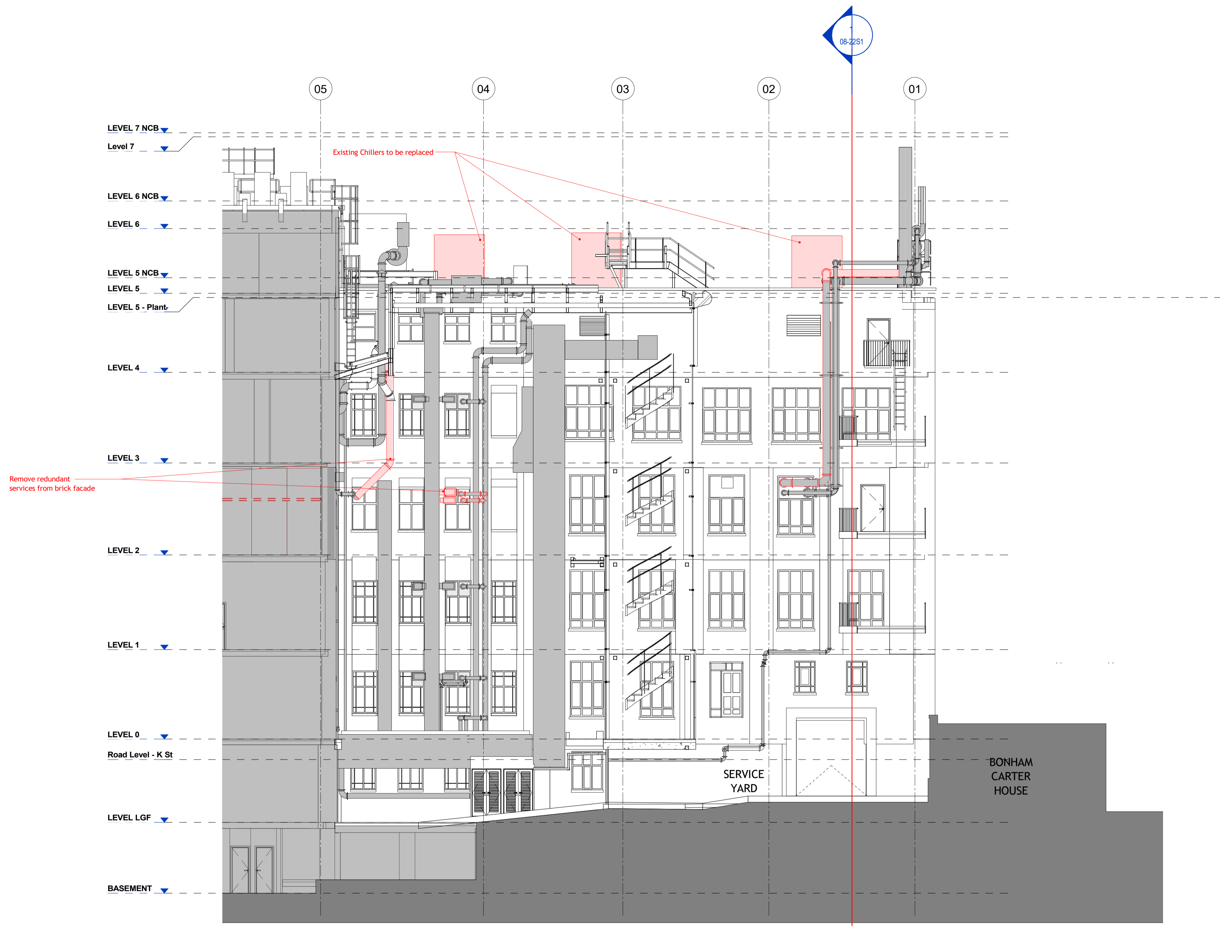
1 Planning Elevation - Existing - NW Wing East Elevation 1 : 100
