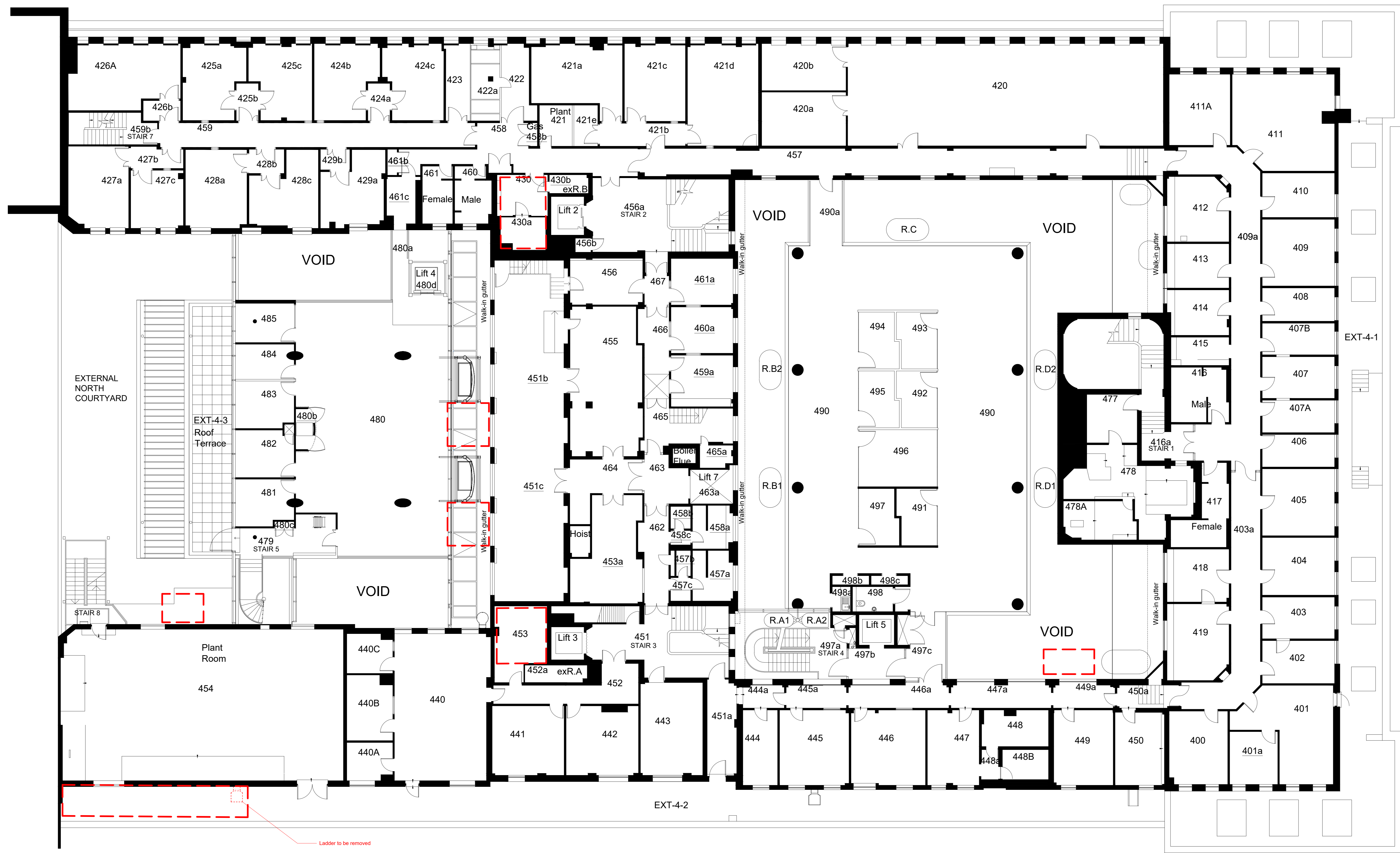
01 Existing Level 04 Plan 08-1804 Scale = 1:100
