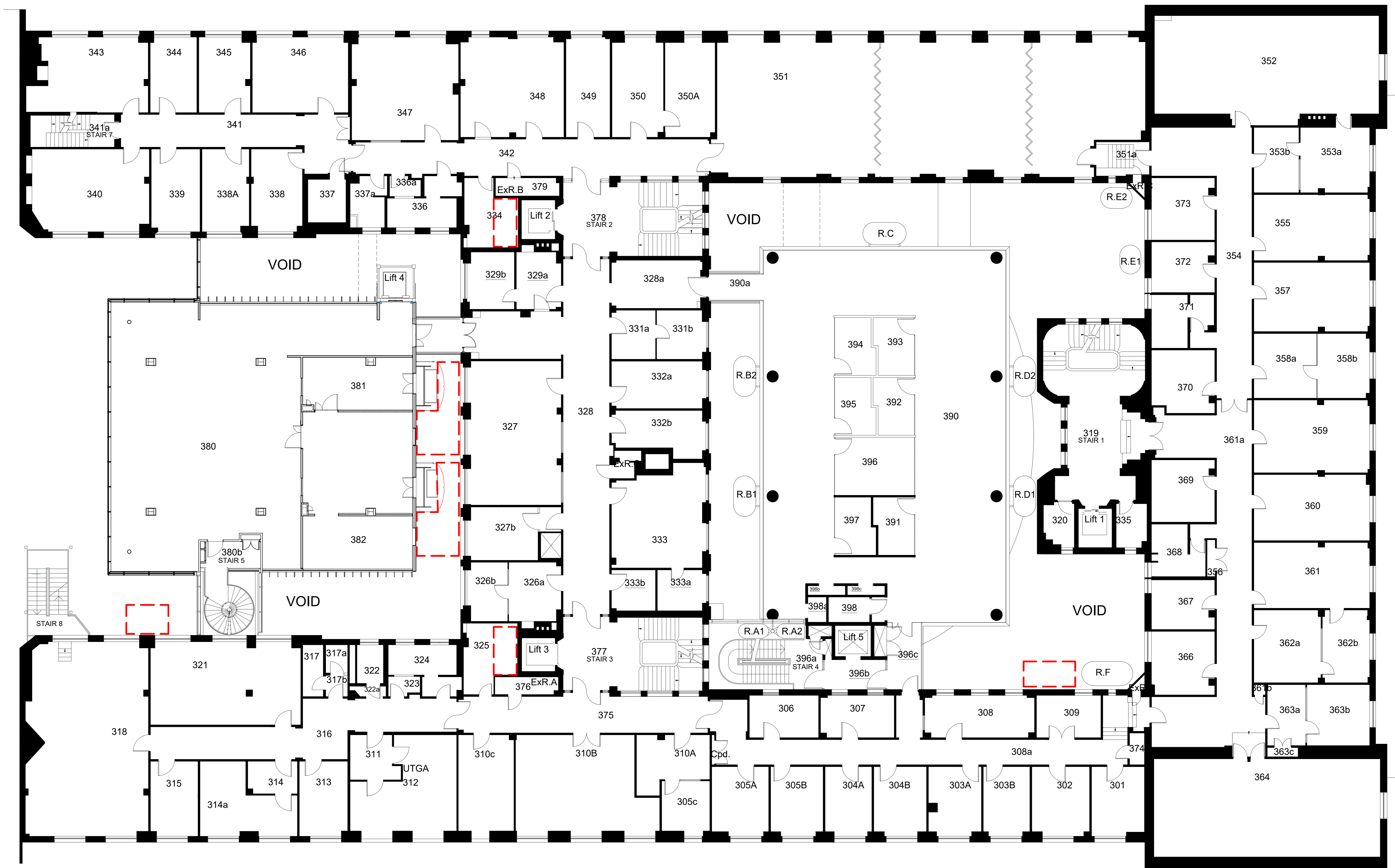
01 Existing Level 03 Plan 08-1803 Scale = 1:100
