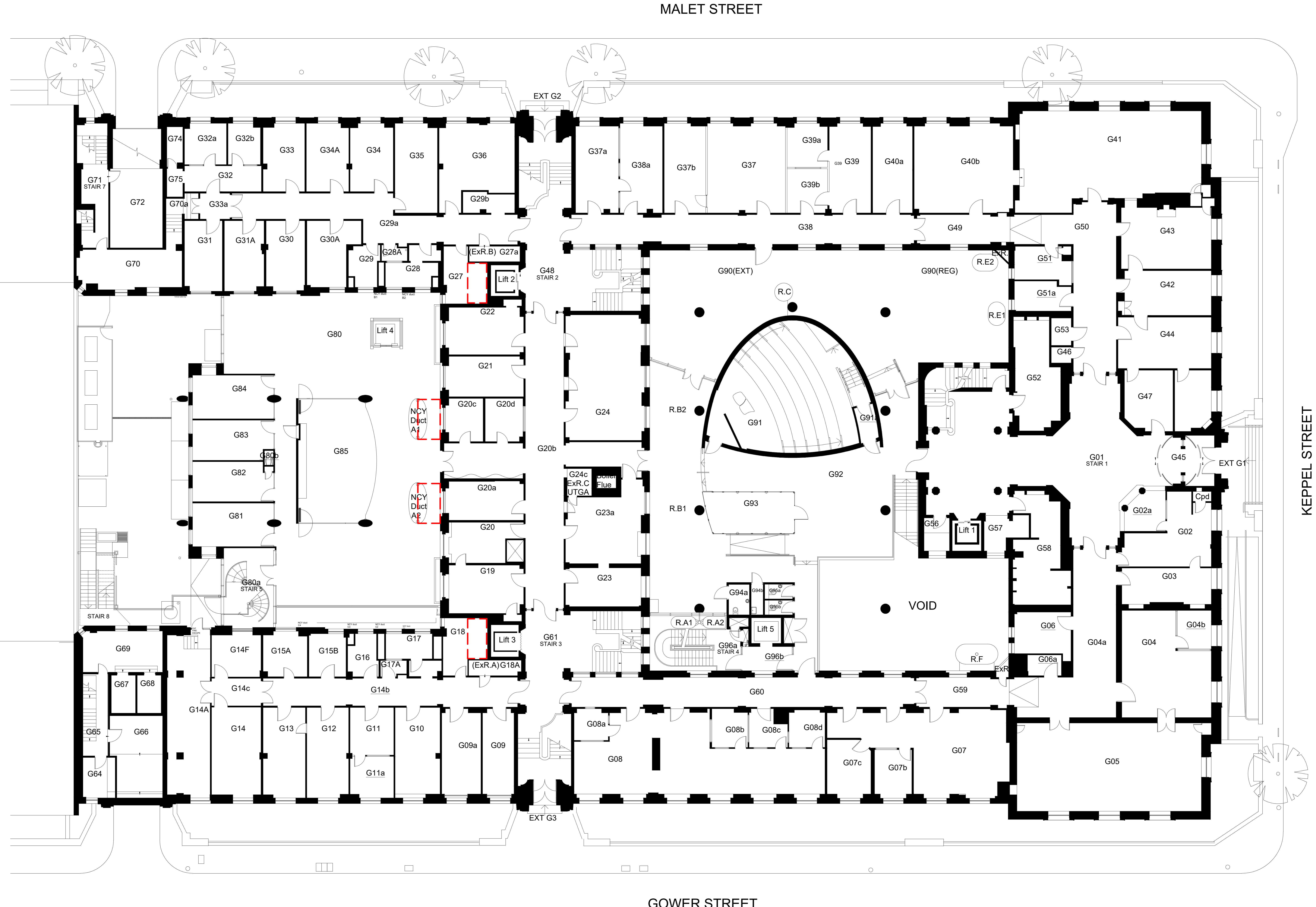
01 Existing Ground Floor Level Plan 08-1800 Scale = 1:100
