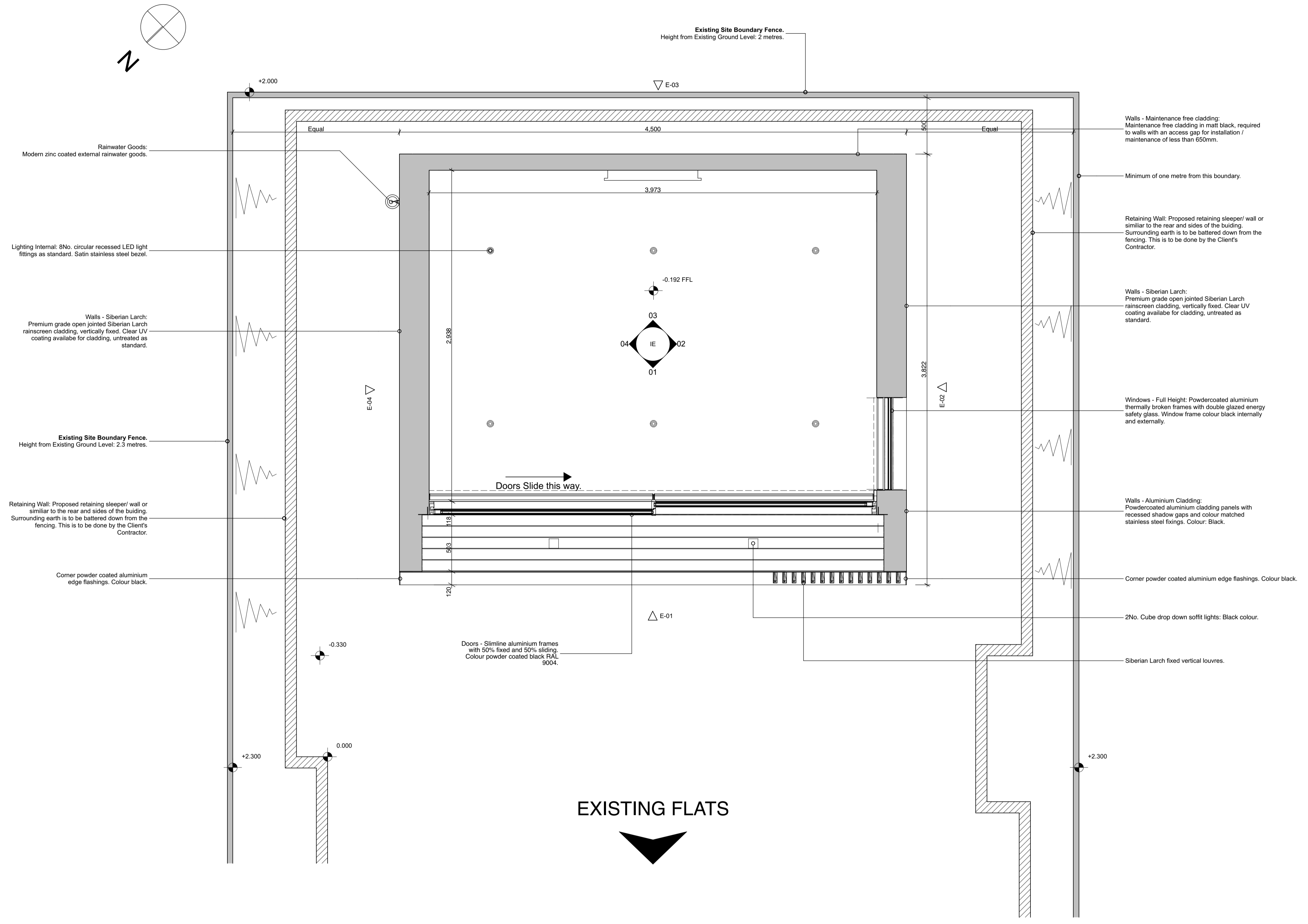
0. GA Ground Floor Plan 1:20
