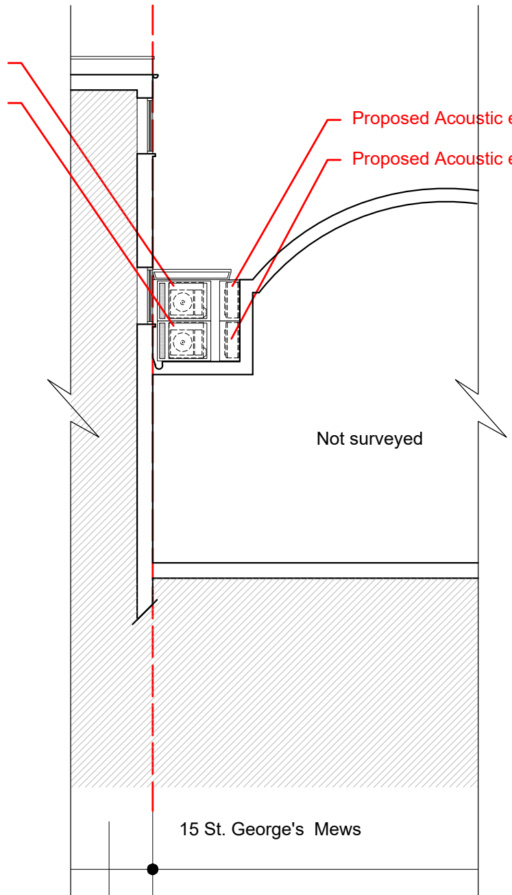
Section BB'
