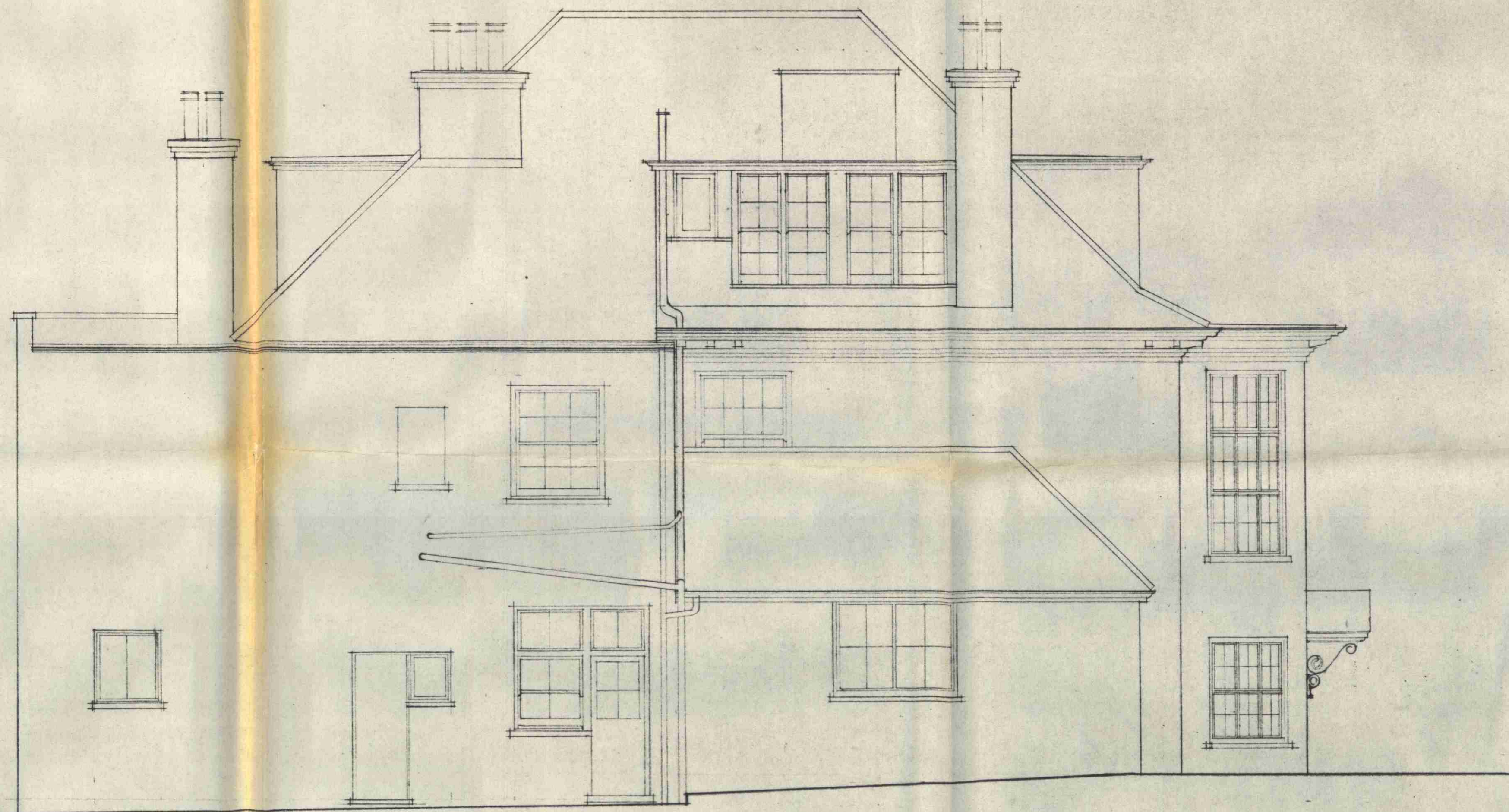
NORTH ELEVATION
