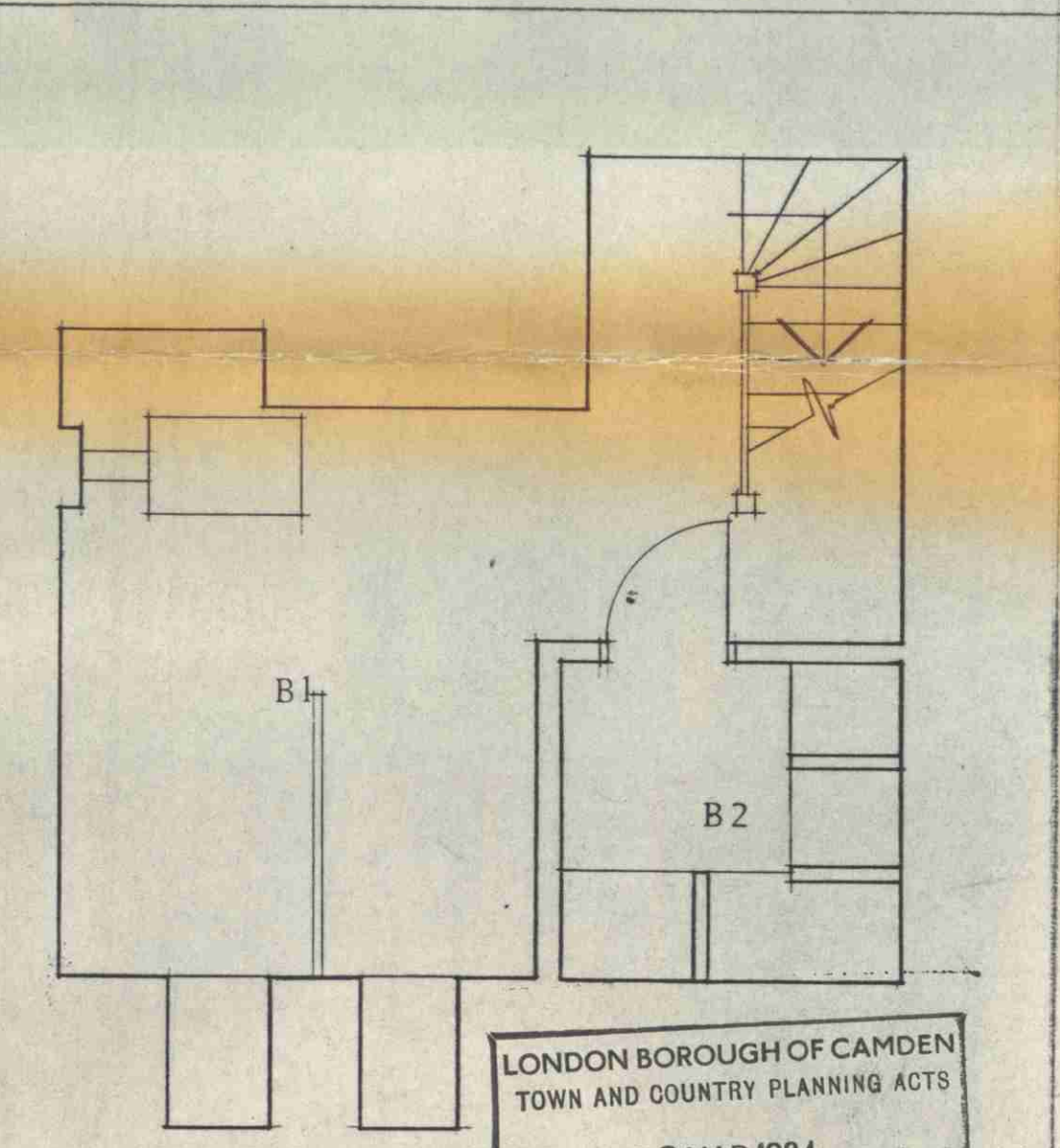
BASEMENT PLAN
