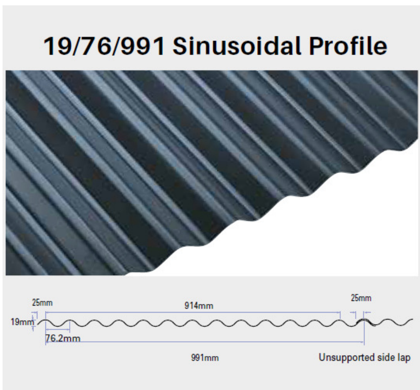
Fig 5 – Corrugated metal cladding sizes
