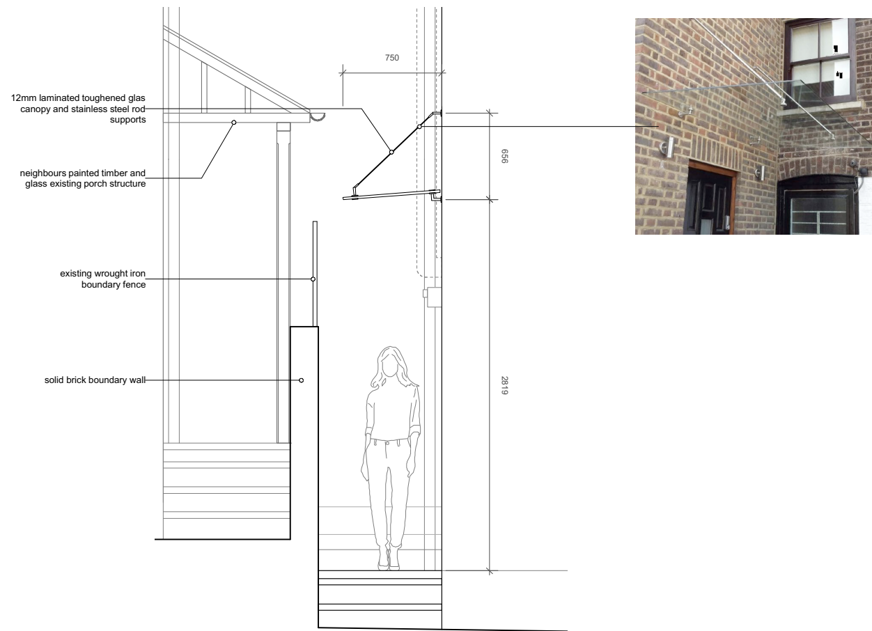
4. CANOPY DETAIL 1:20 @ A1
