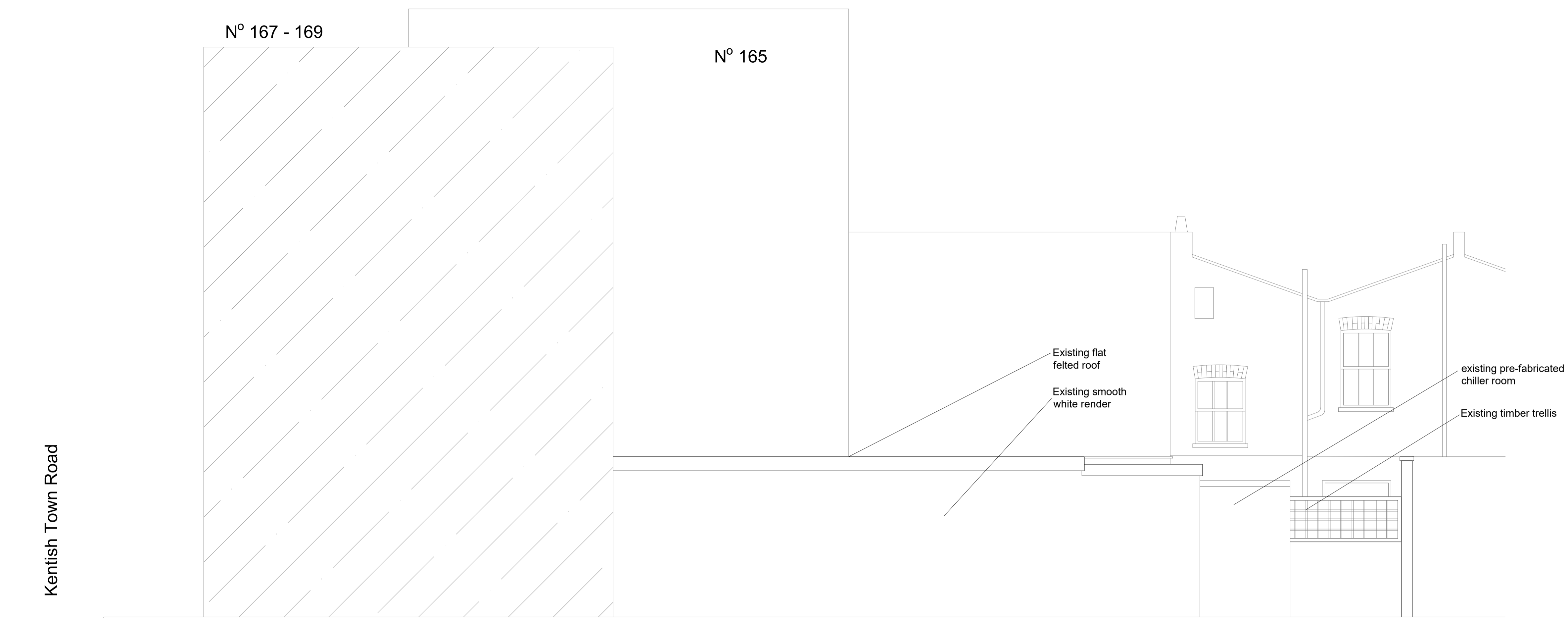
Existing Side Elevation Elevation Facing N°165 Scale 1:50 @ A1
