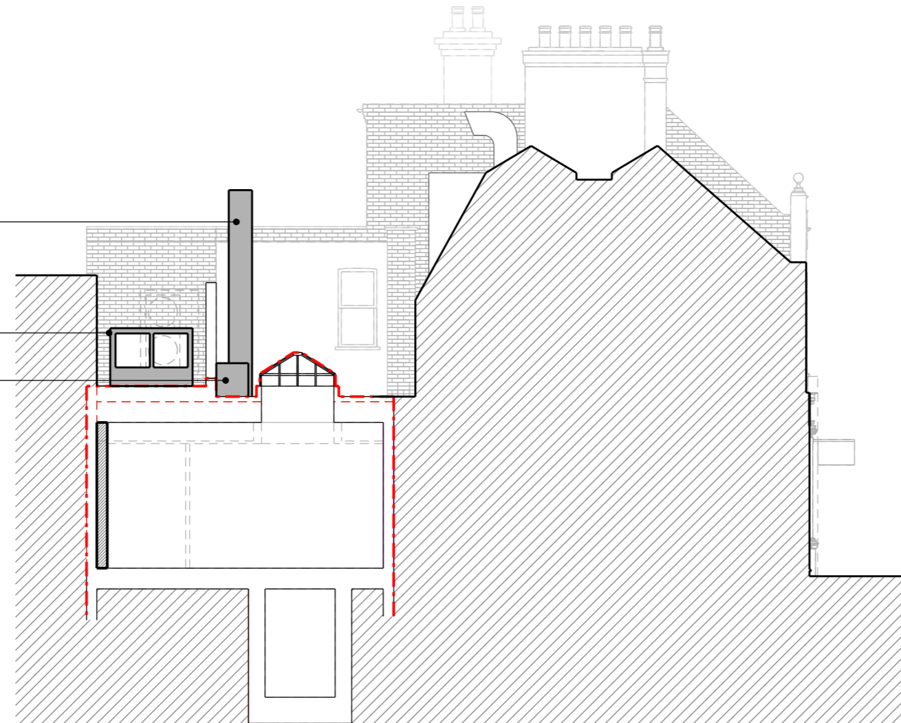
Proposed Sectional Elevation B-B
