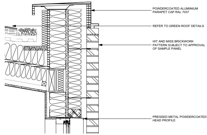
1 PARAPET DETAIL OF BRICK PANELS
