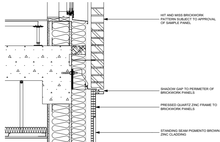
2 BASE OF BRICKWORK DETAIL
