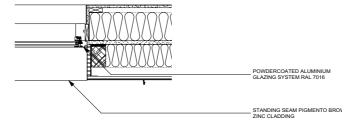
7 GROUND FLOOR WINDOW JAMB DETAIL
