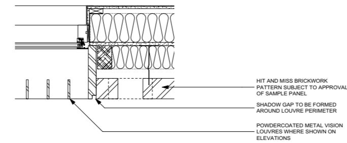
5 PLAN DETAIL OF VISION SCREEN AT JAMB
