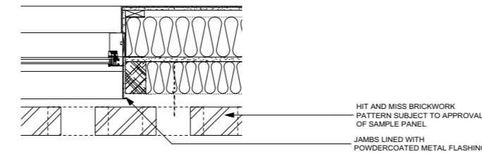
6 PLAN DETAIL OF WINDOW CONCEALED BEHIND BRICKWORK
