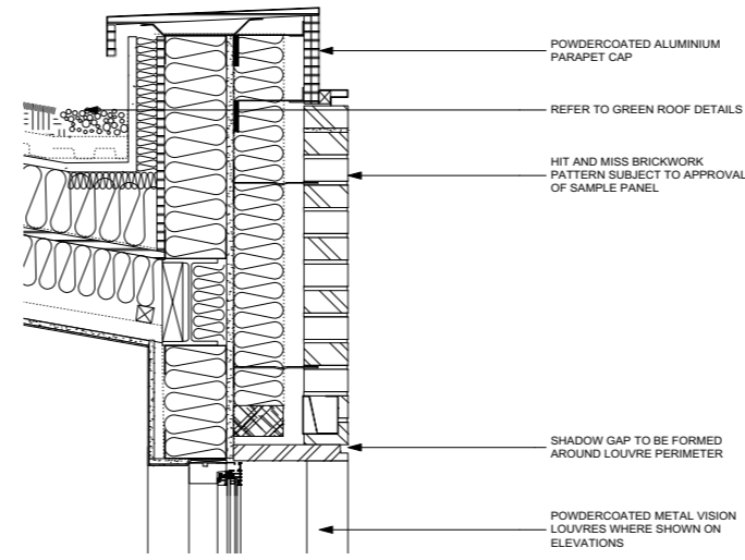
4 PARAPET DETAILED SECTION THROUGH WINDOW LOUVRE
