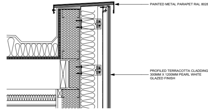
7 PARAPET DETAIL AT TERRECOTTA CLADDING
