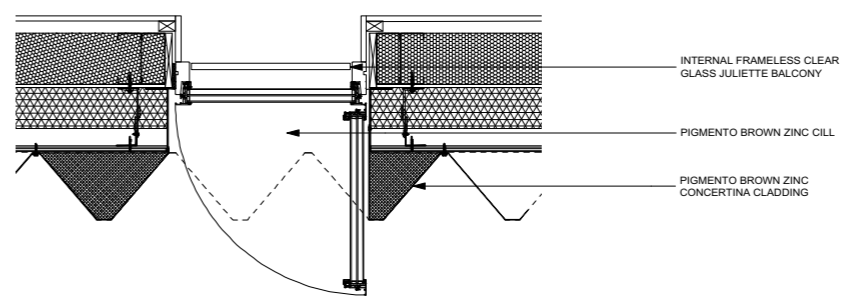
12 PLAN SECTION OF WINDOW SOUTHERN ELEVATION
