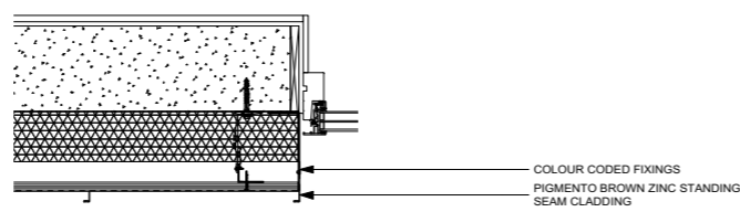
9 WINDOW JAMB DETAIL STANDING SEAM
