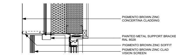
2 WINDOW HEAD DETAIL
