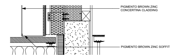
6 BASE DETAIL
