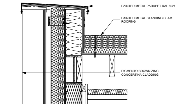
1 PARAPET DETAIL
