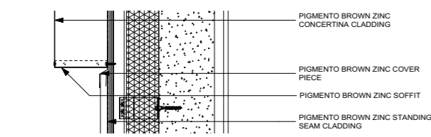
4 JUCTION DETAIL CONCERTINA CLADDING AND STANDING SEAM
