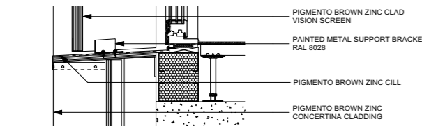
3 WINDOW CILL DETAIL
