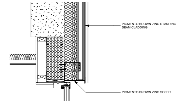
8 WINDOW HEAD DETAIL STANDING SEAM
