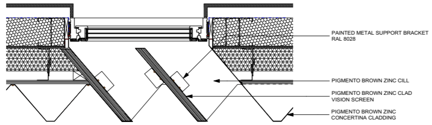
10 PLAN SECTION OF WINDOW LOUVRE
