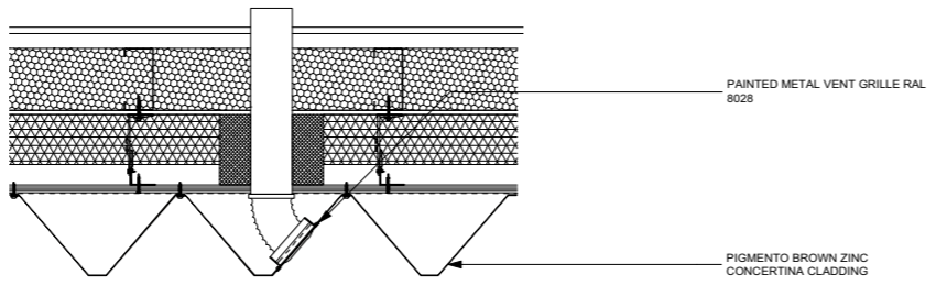
11 VENTILATION GRILLE DETAIL
