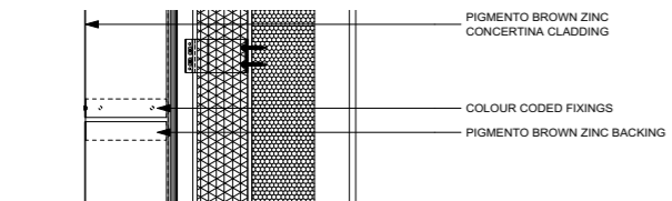
5 BUTT JOINT DETAIL
