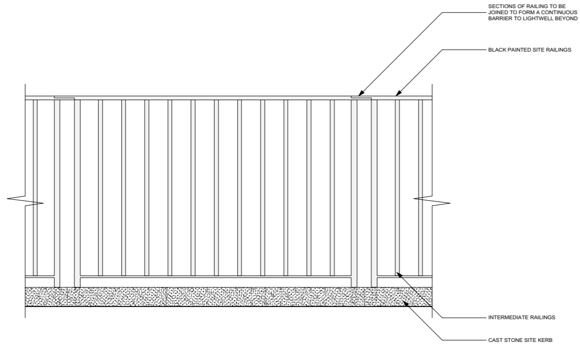
1 ELEVATION OF SITE RAILINGS
