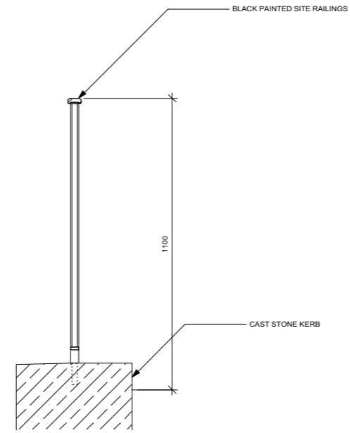
2 SECTION THROUGH RAILING
