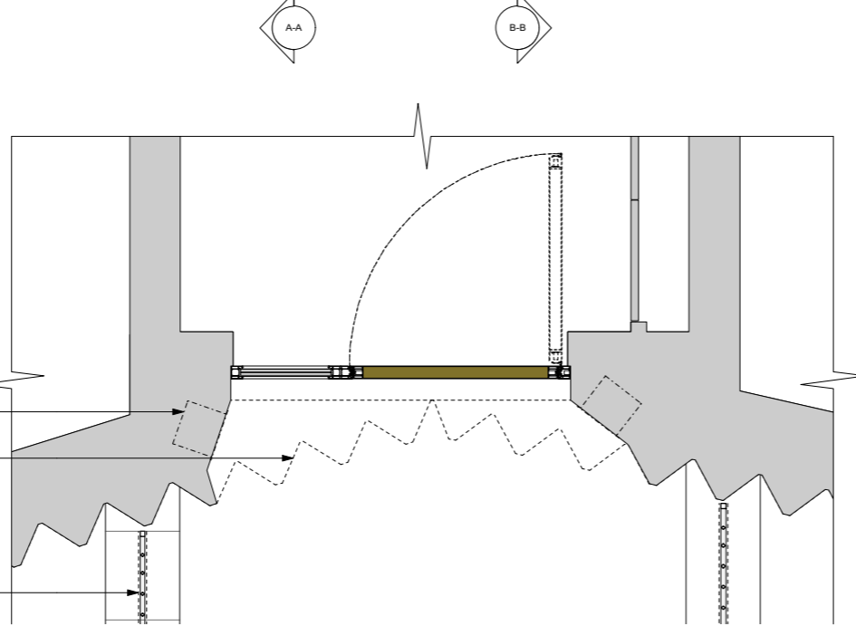
4 PARTIAL PLAN
