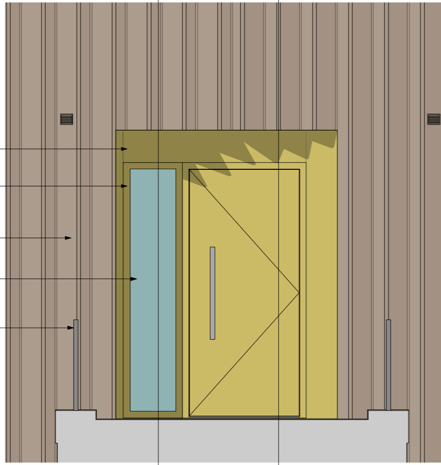
2 PARTIAL REAR ELEVATION
