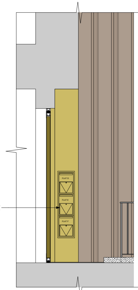
3 SECTION B-B
