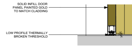
8 DOOR THRESHOLD DETAIL Scale: 1:10
