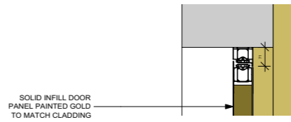
7 DOOR HEAD DETAIL Scale: 1:10
