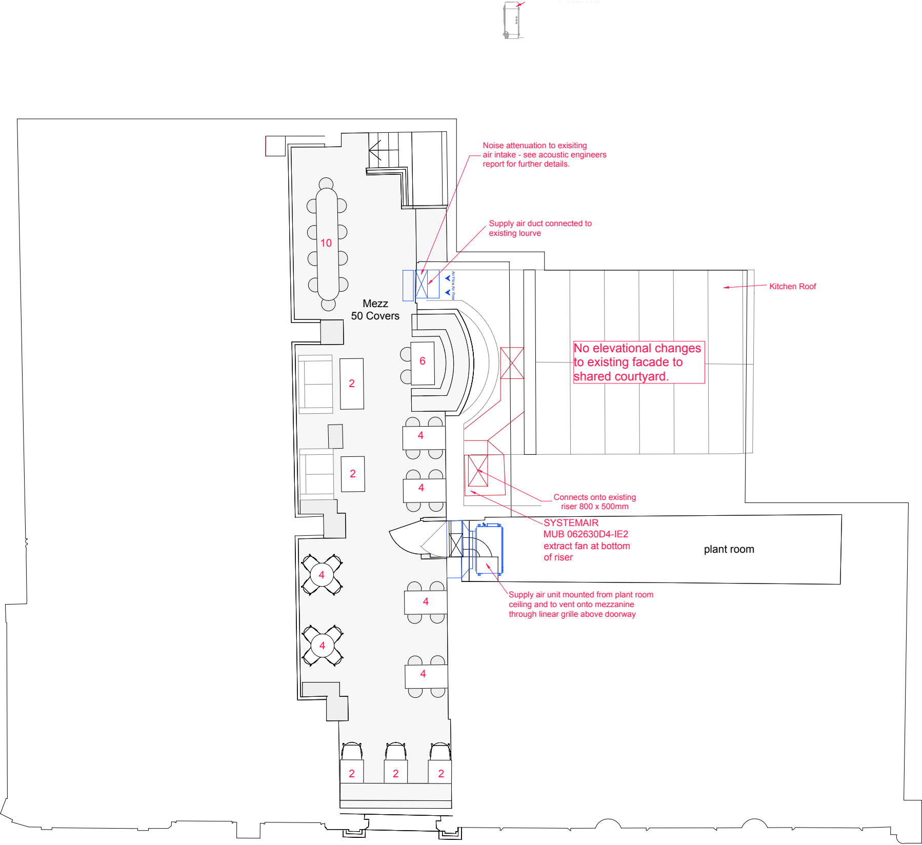
02 Mezzanine Furniture Layout - Proposed 1:100
