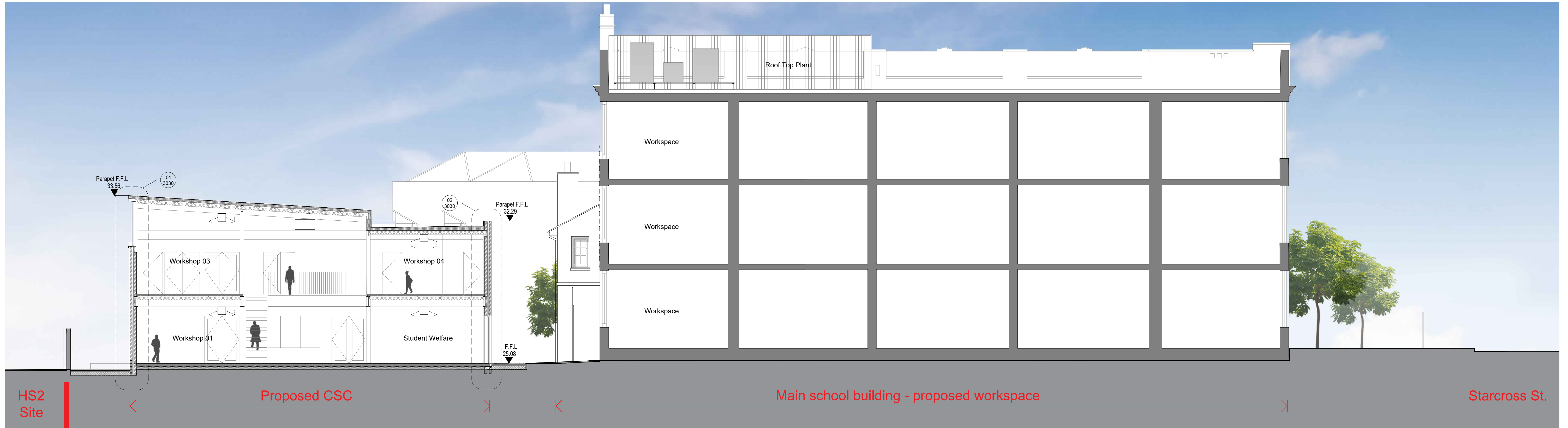
02 Section B-B
