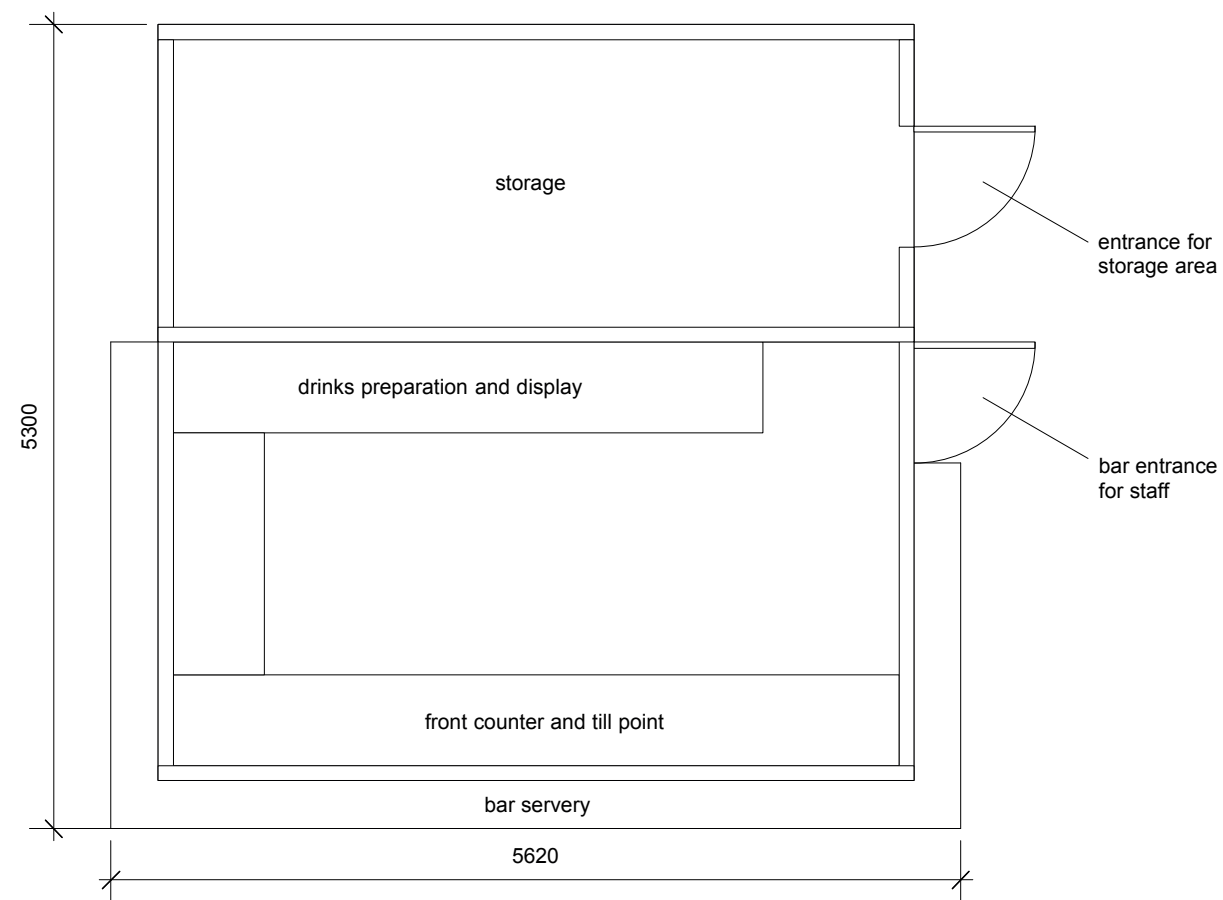
PLAN VIEW WITHOUT ROOF
