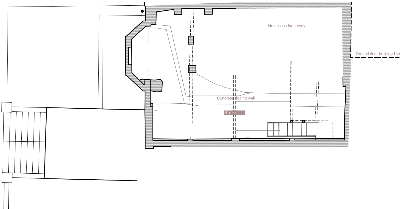
Existing Lower Ground Floor Plan - 1:100@A3
