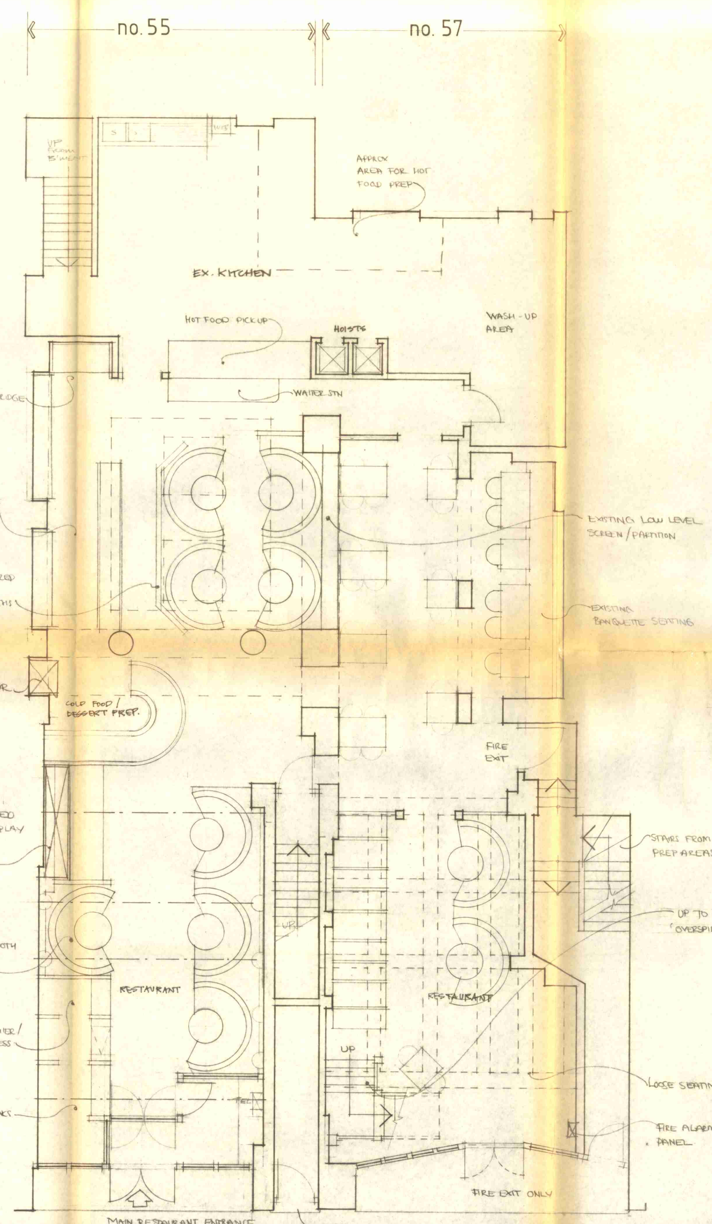
Ground Floor Plan (NO 55 ONLY)
