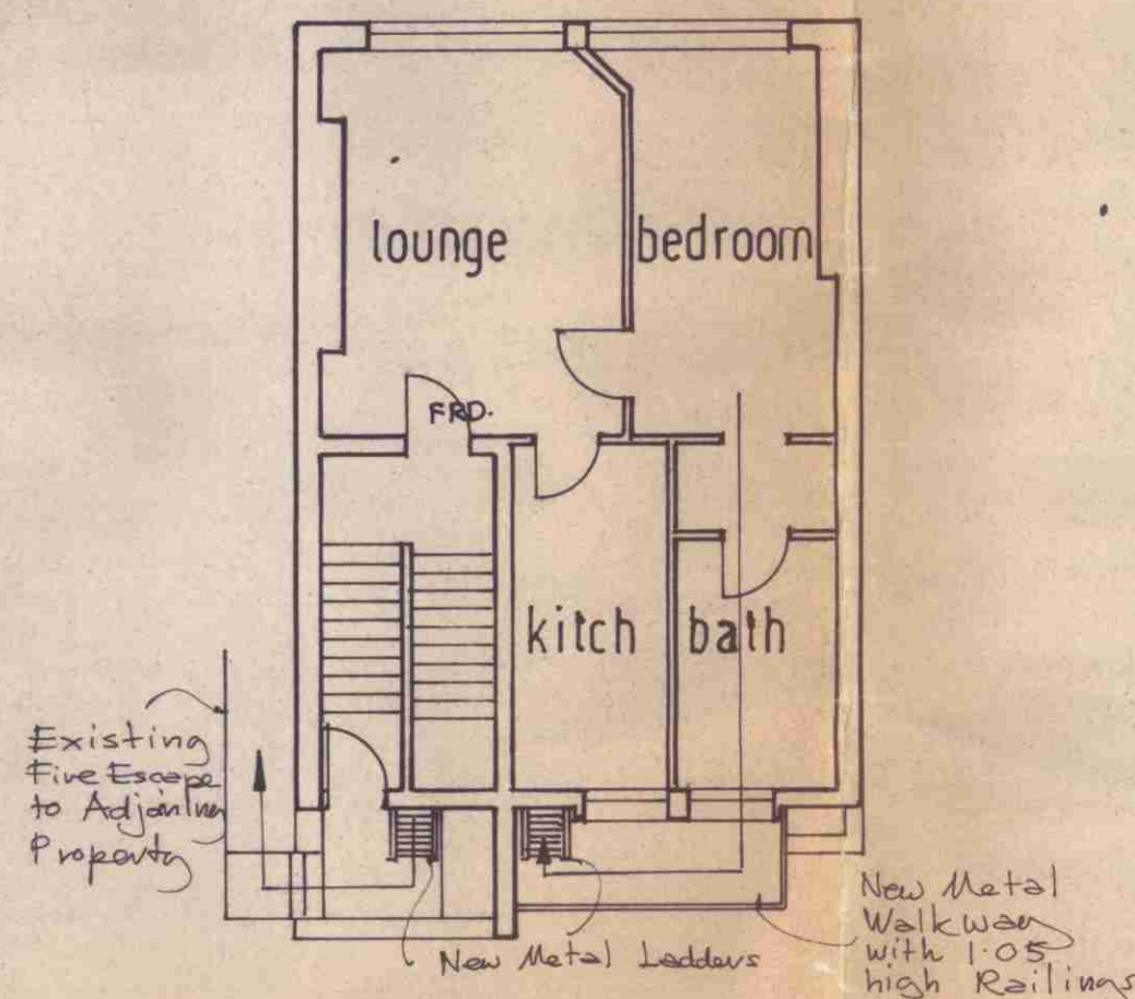
5th FLOOR PLAN SHOWING PROPOSED FIRE ESCAPE
