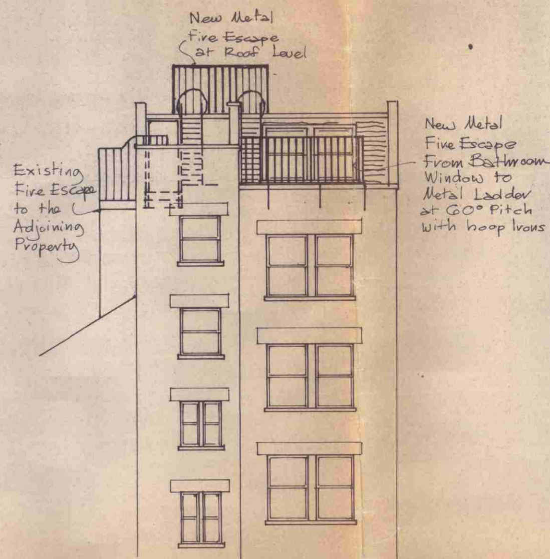
REAR ELEVATION SHOWING PROPOSED FIRE ESCAPE
