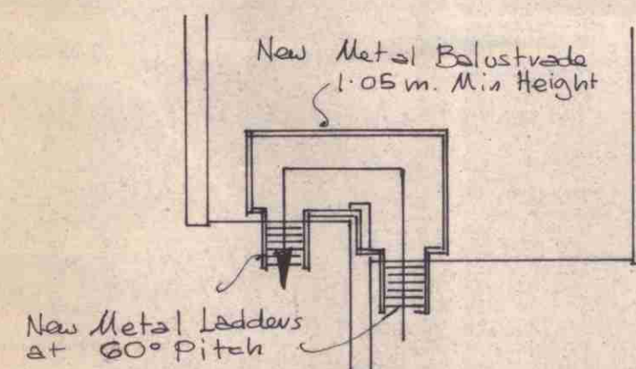
PART ROOF PLAN SHOWING PROPOSED ESCAPE ROUTE
