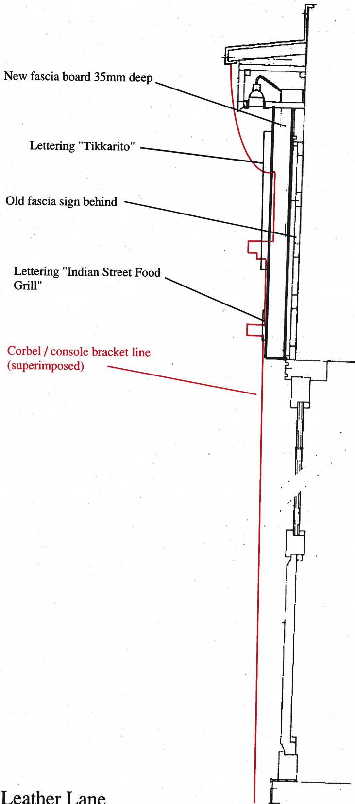
Drawing 1: Section drawing
