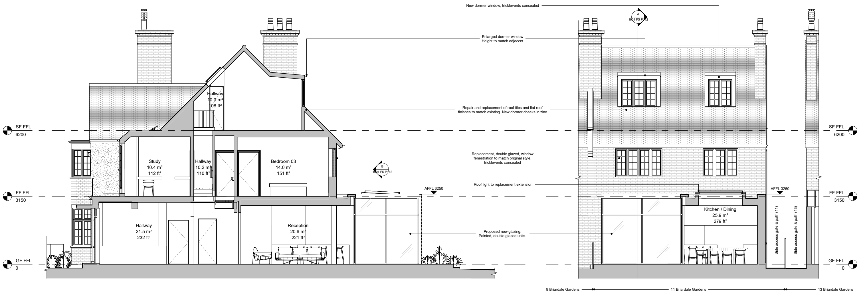
A Proposed - Section A 1 : 50
