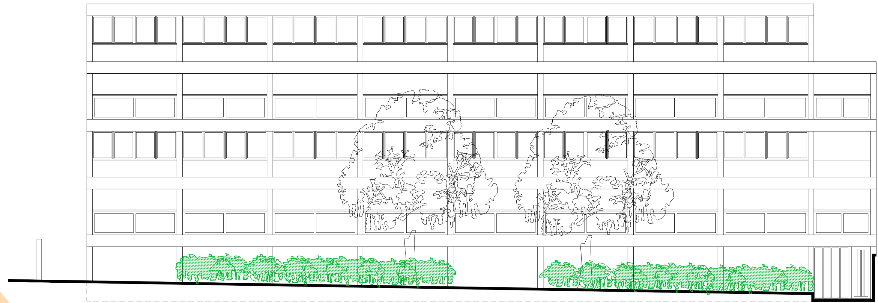
ELEVATION TO CHURCHWAY
