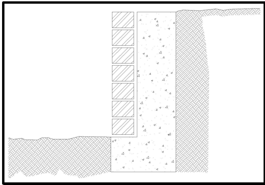
Figure 4: Indicative cross section of a “toe out” type foundation
