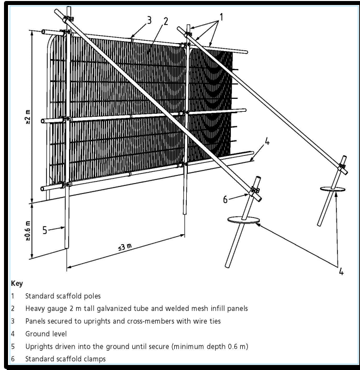
Figure 2: BS5837:2012 - Figure 2, Default specification for protective barriers.
