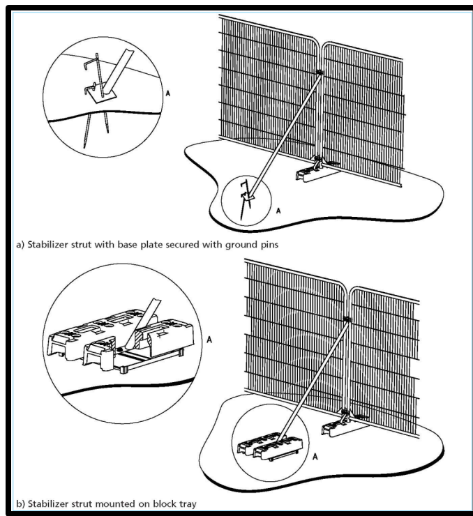
Figure 3: BS5837:2012 - Figure 3, Examples of above-ground stabilising systems.
