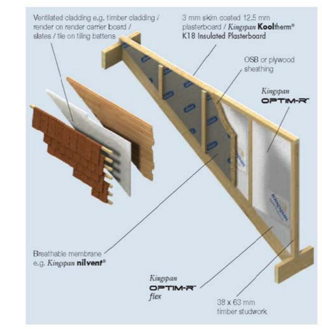
Dormer Cheek
