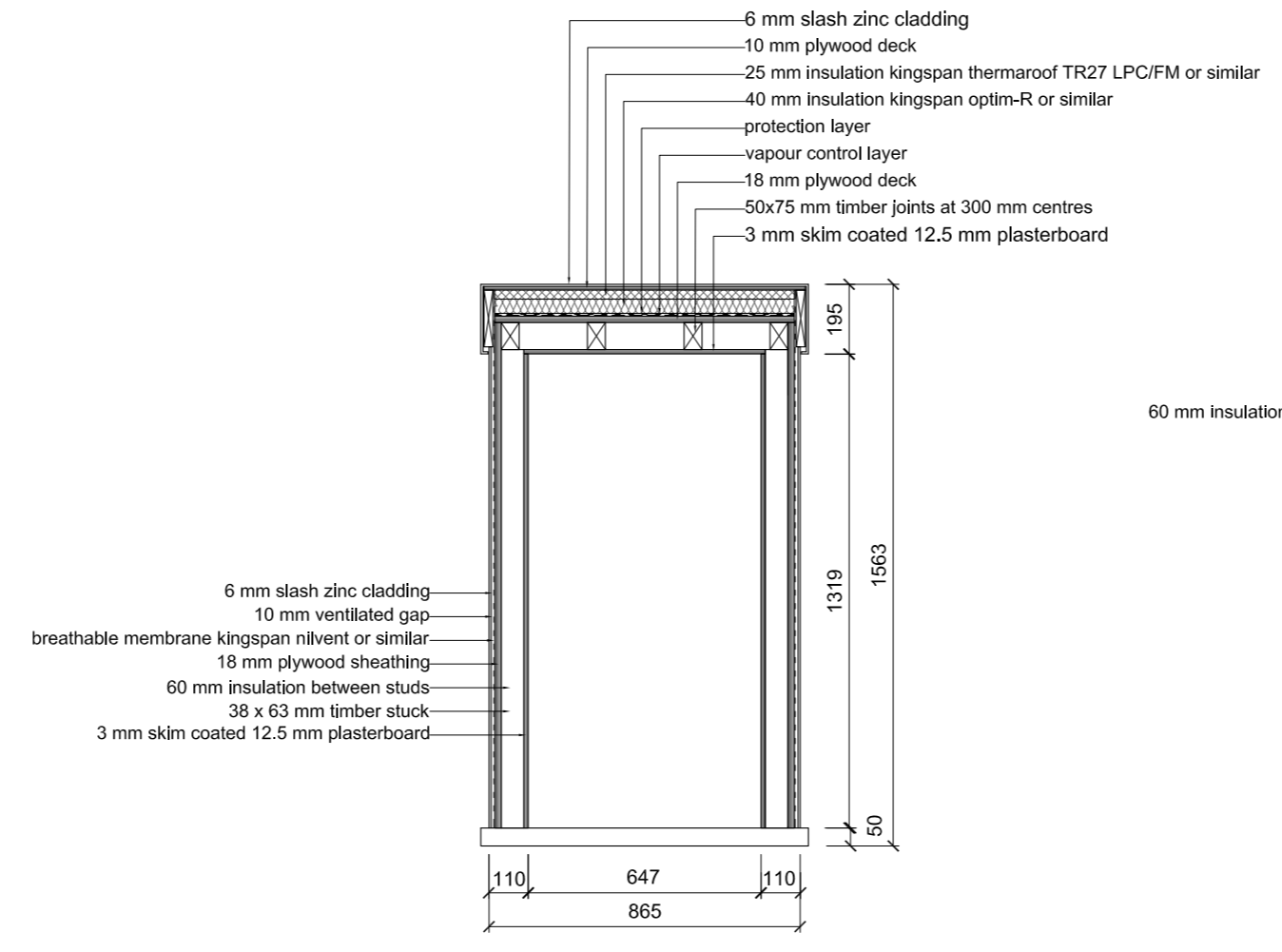
2 DORMER SECTION 1:20@A2
