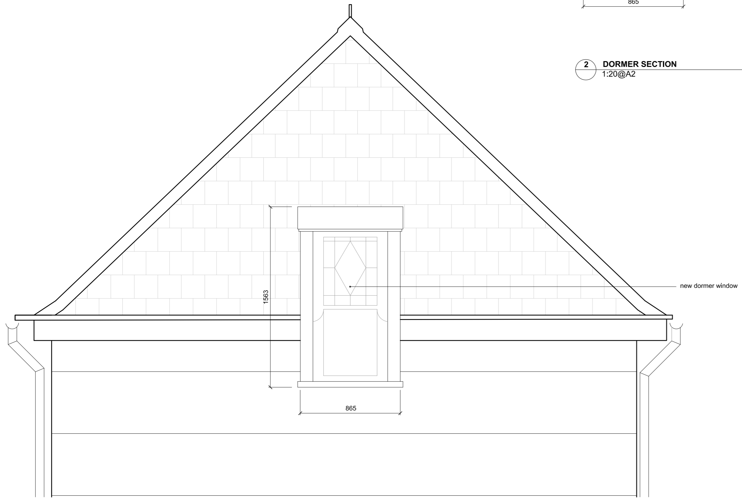
1 REAR ELEVATION 1:20@A2
