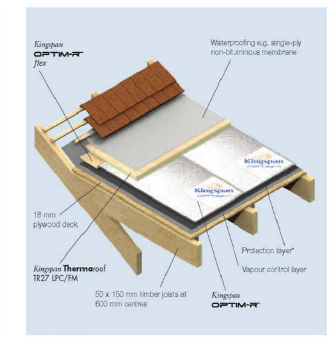
Dormer Roof
