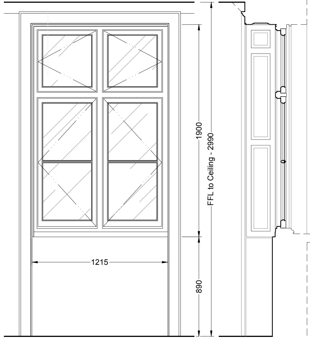
Internal Elevation 1:20
