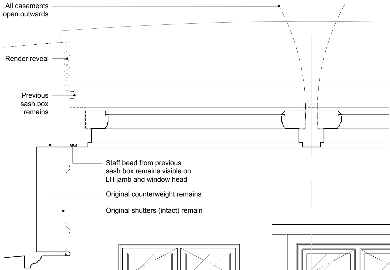
Jamb/Meeting Stile Detail 1:5
