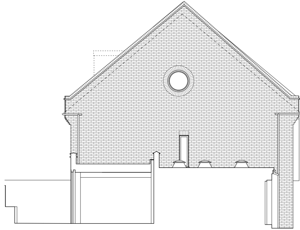
2 SIDE ELEVATION
