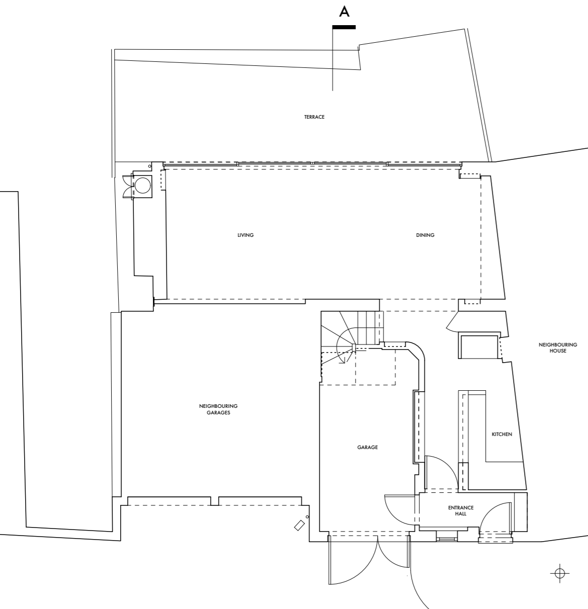
5 GROUND FLOOR PLAN
