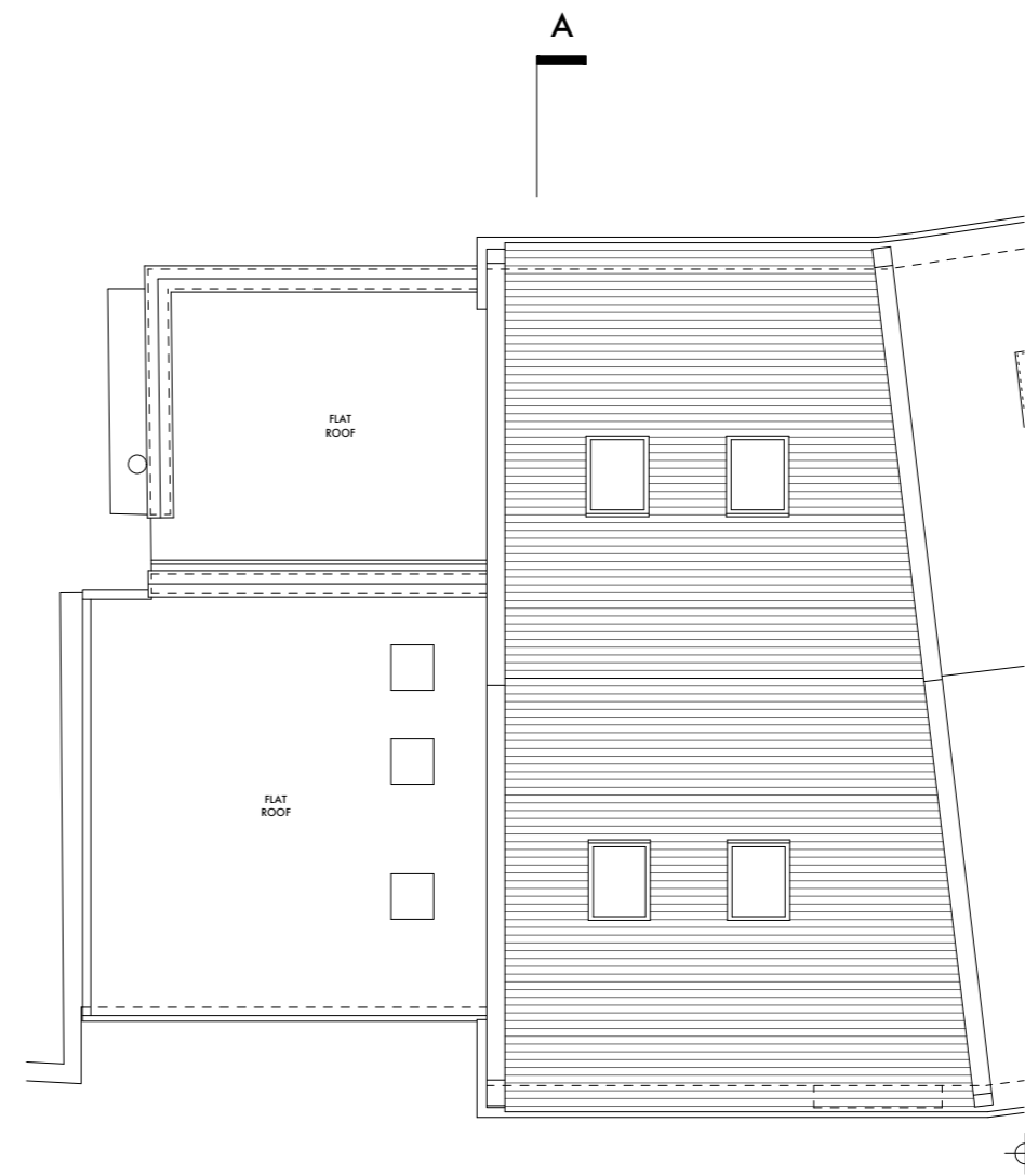
7 ROOF PLAN
