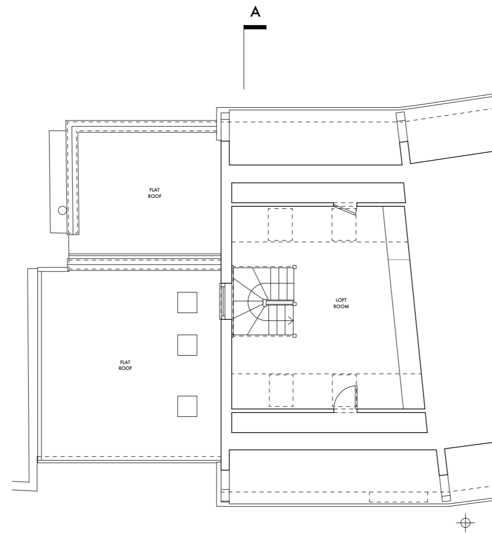
6 SECOND FLOOR PLAN
