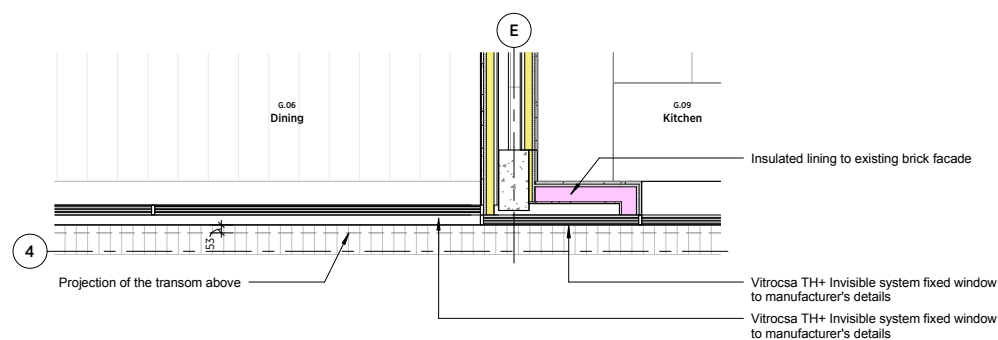
4 GROUND FLOOR TYPICAL WINDOW PLAN 1:25
