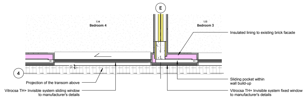
3 FIRST FLOOR TYPICAL WINDOW PLAN 1:25
