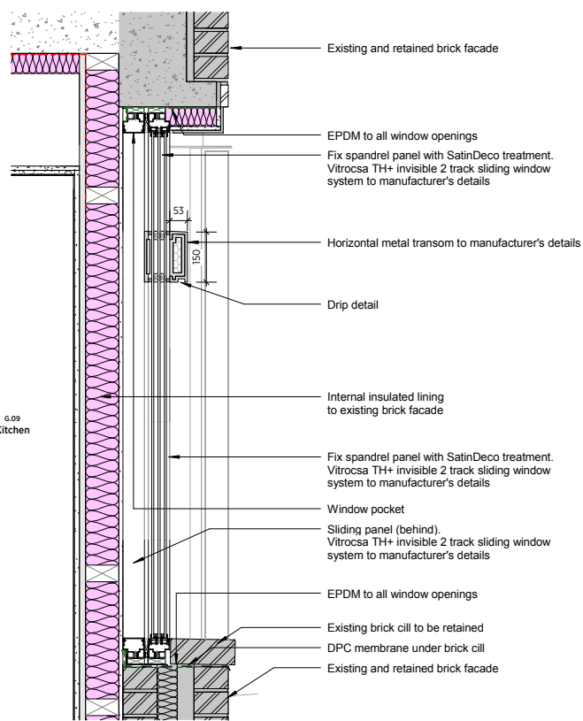
1 TYPICAL WINDOW SPANDREL DETAIL - GROUND AND FIRST FLOORS 1:10
