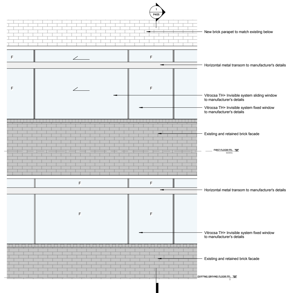
2 EXTRACT OF FRONT FACADE WINDOW ELEVATION 1:25
