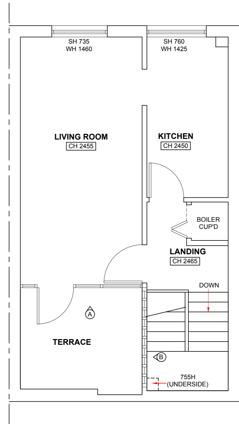
UPPER FLOOR
