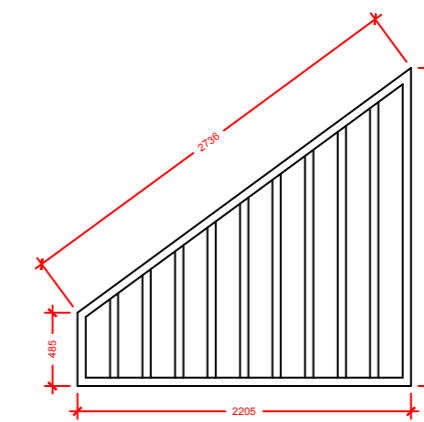
WINDOW DETAIL B
