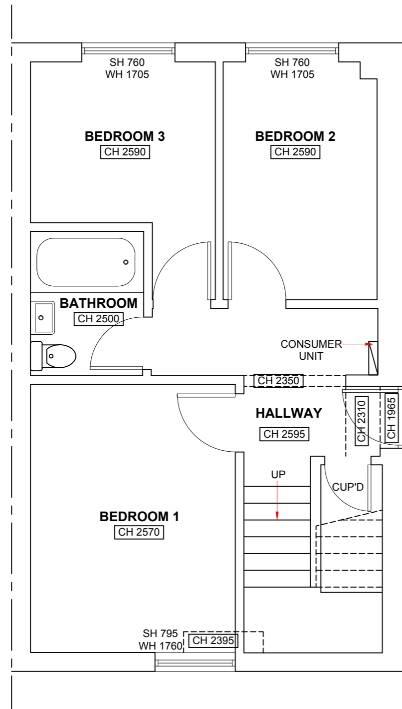
LOWER FLOOR
