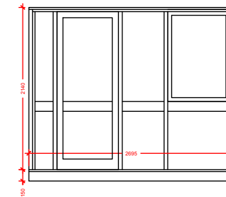
WINDOW DETAIL A
