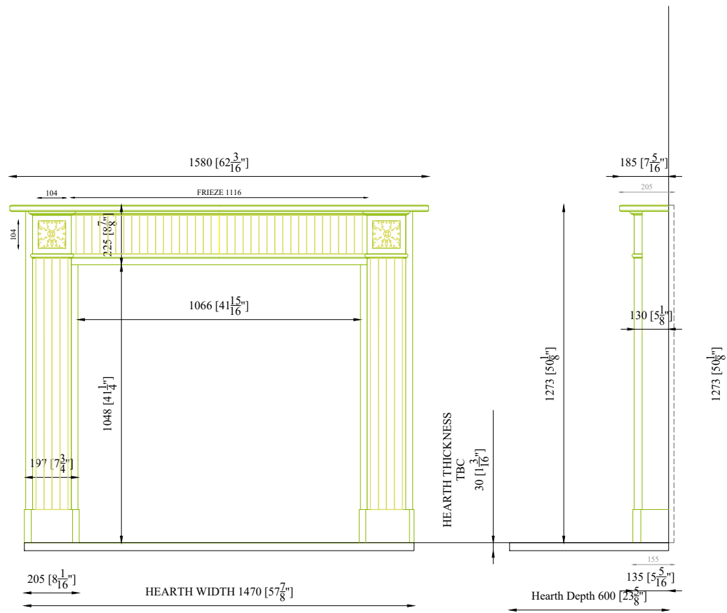
FRONT ELEVATION
