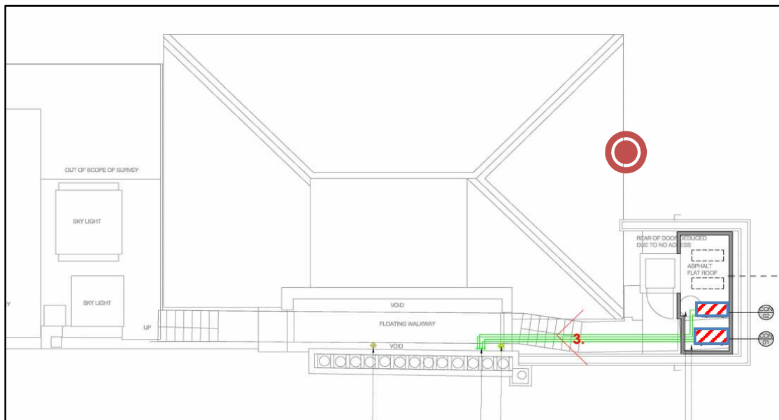
Figure 2.2 Site measurement position and proposed pant unit installation (Drawing Source: WOW Architects)
