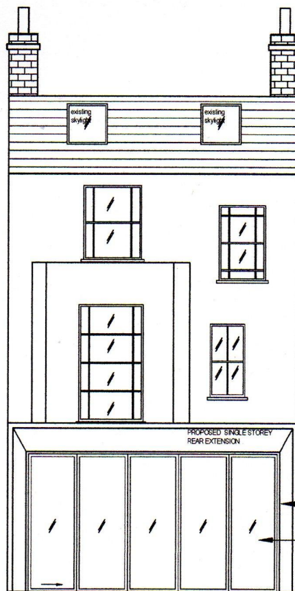
BACK ELEVATION
