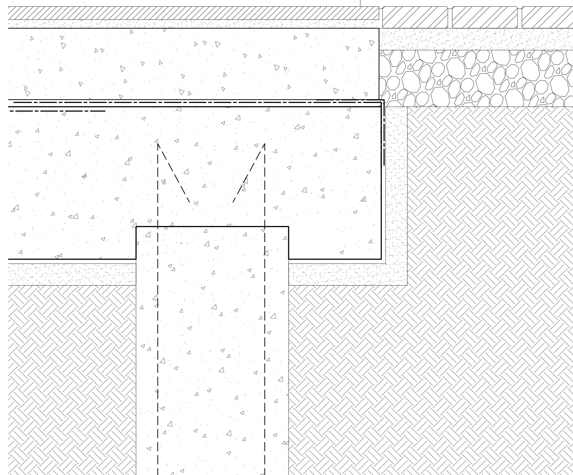
DETAIL DD-146 SECTION AA
