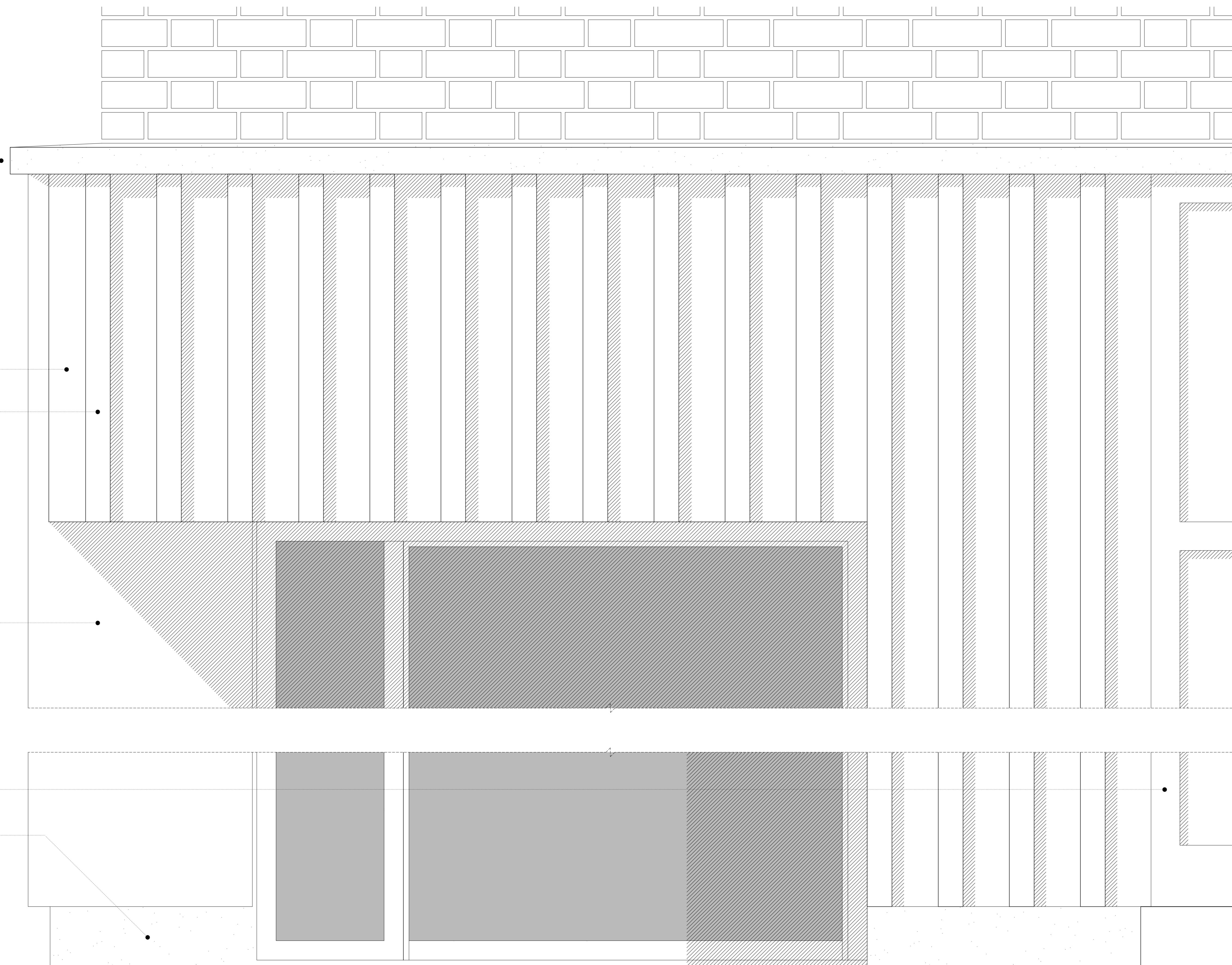
DETAIL DD-146 ELEVATION
