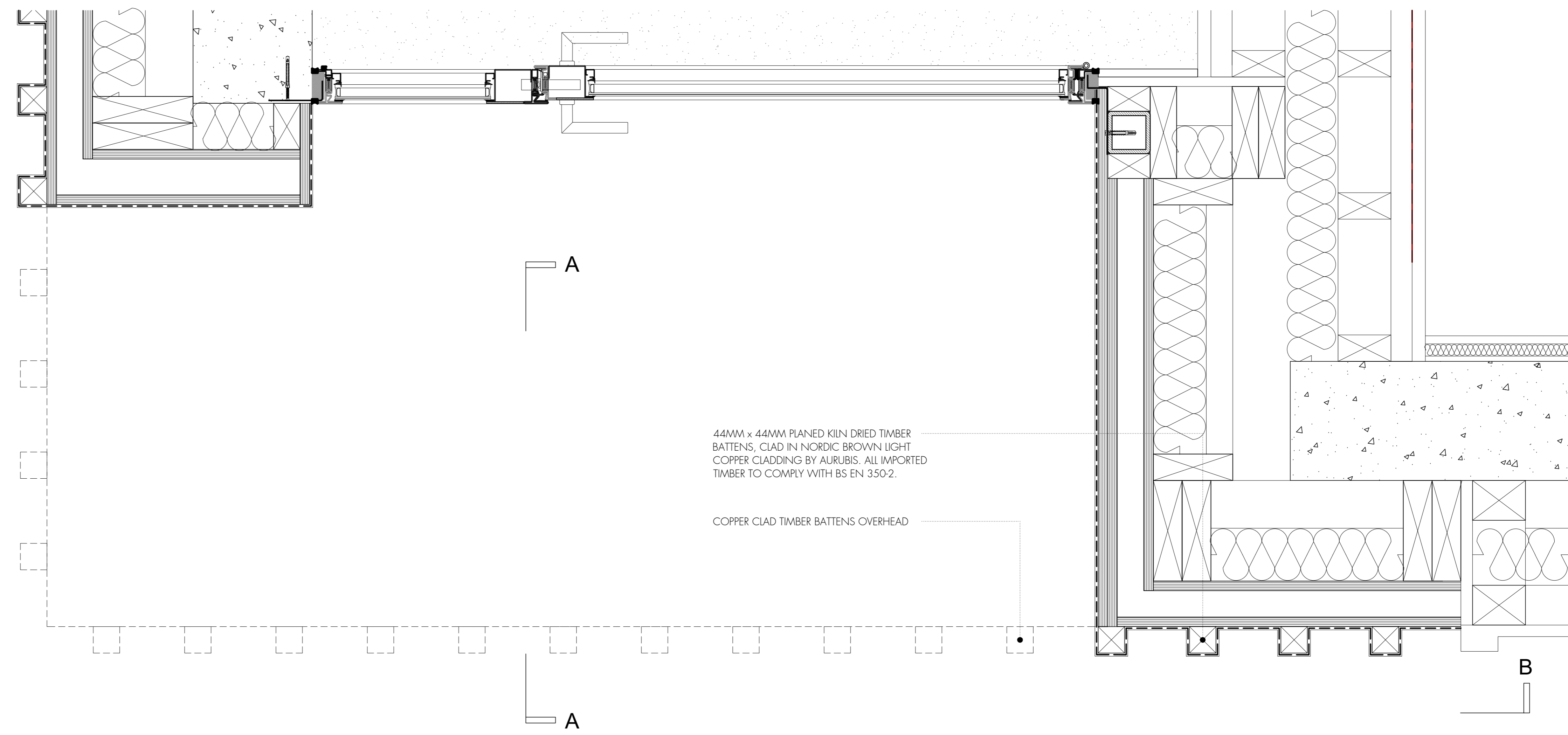
DETAIL DD-146 PLAN
