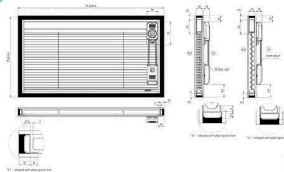
SL20C Venetian and SL20C Pleated
