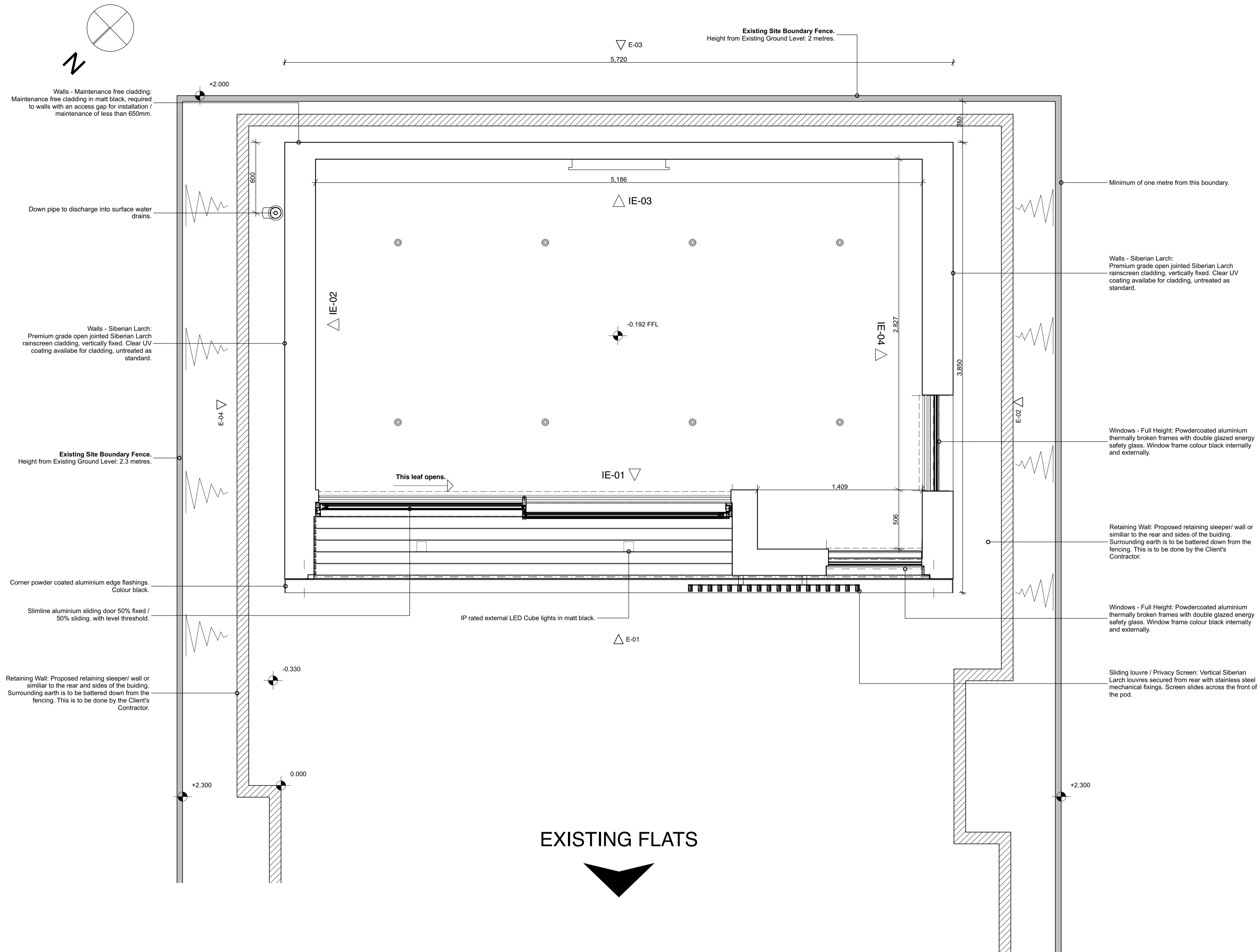
0. GA Ground Floor Plan 1:20
