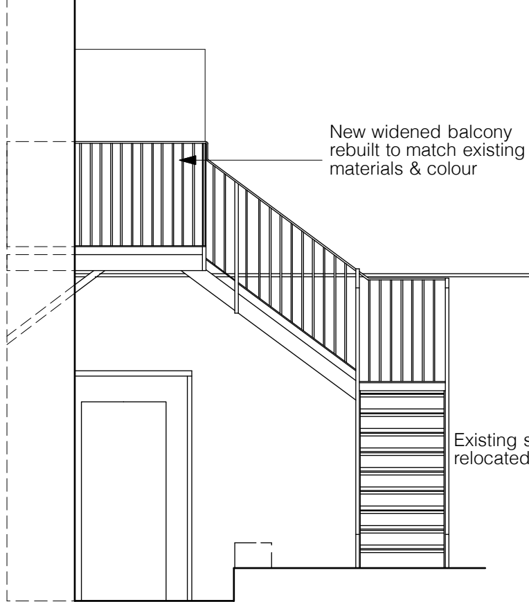
Proposed Side Elevation 1
