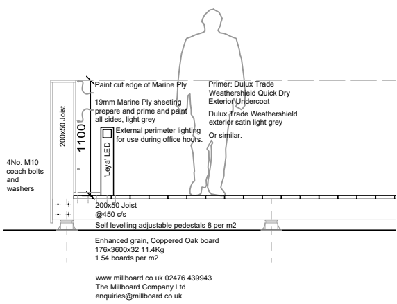
Section through terrace edge: 1/50 SEE ALSO: D/02
