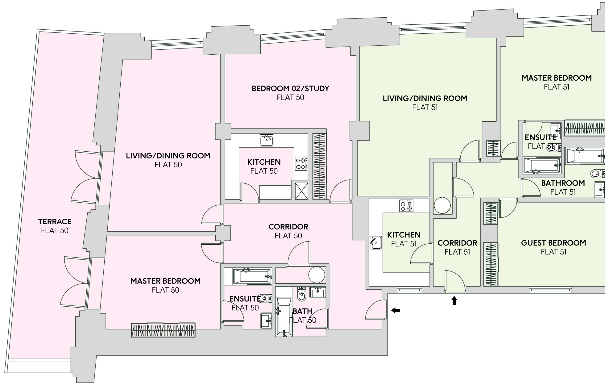
EXISTING FLOOR PLAN 1:100 Flat 50 & 51 Gilbey House
