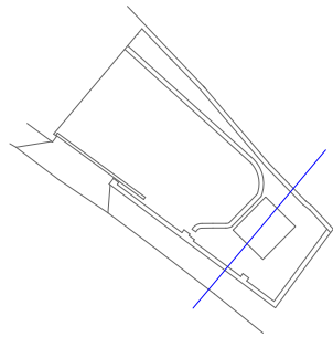
EXISTING SECTION AA 1:50
