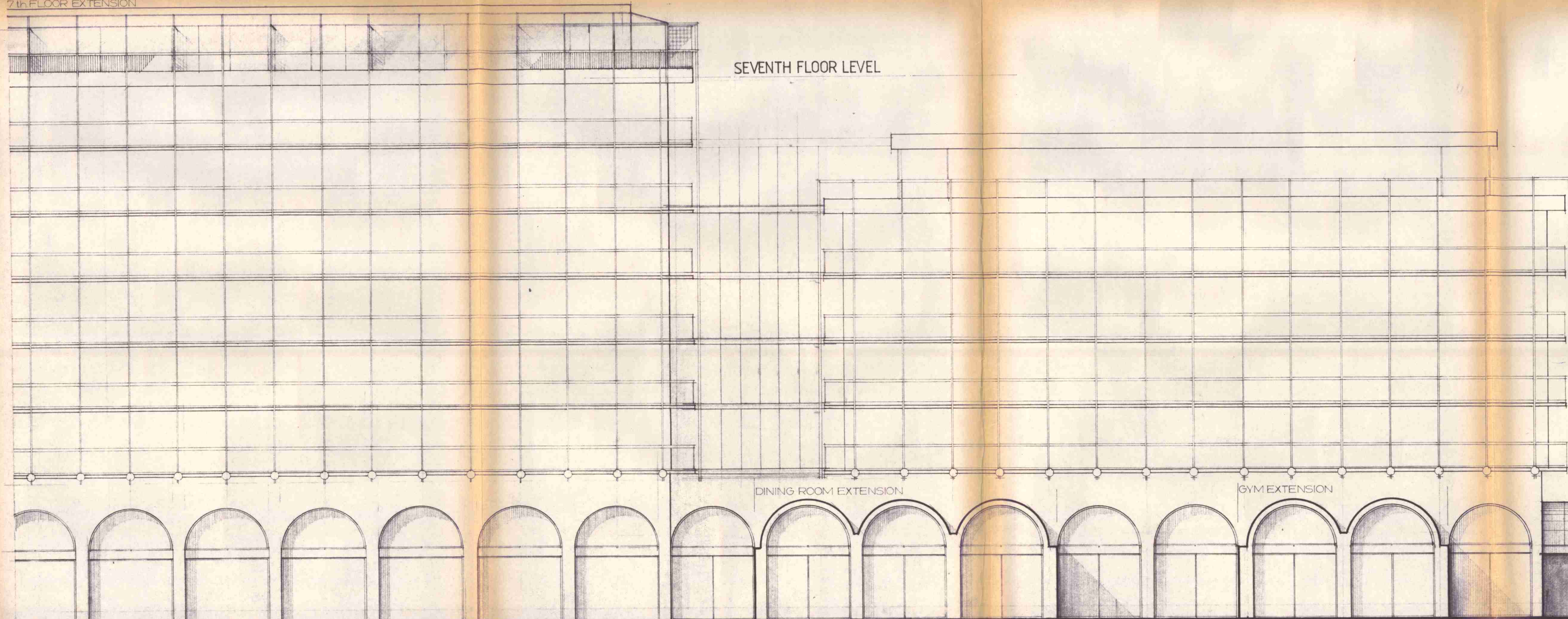
PROPOSED ELEVATION (C) ADELAIDE ROAD NORTH
